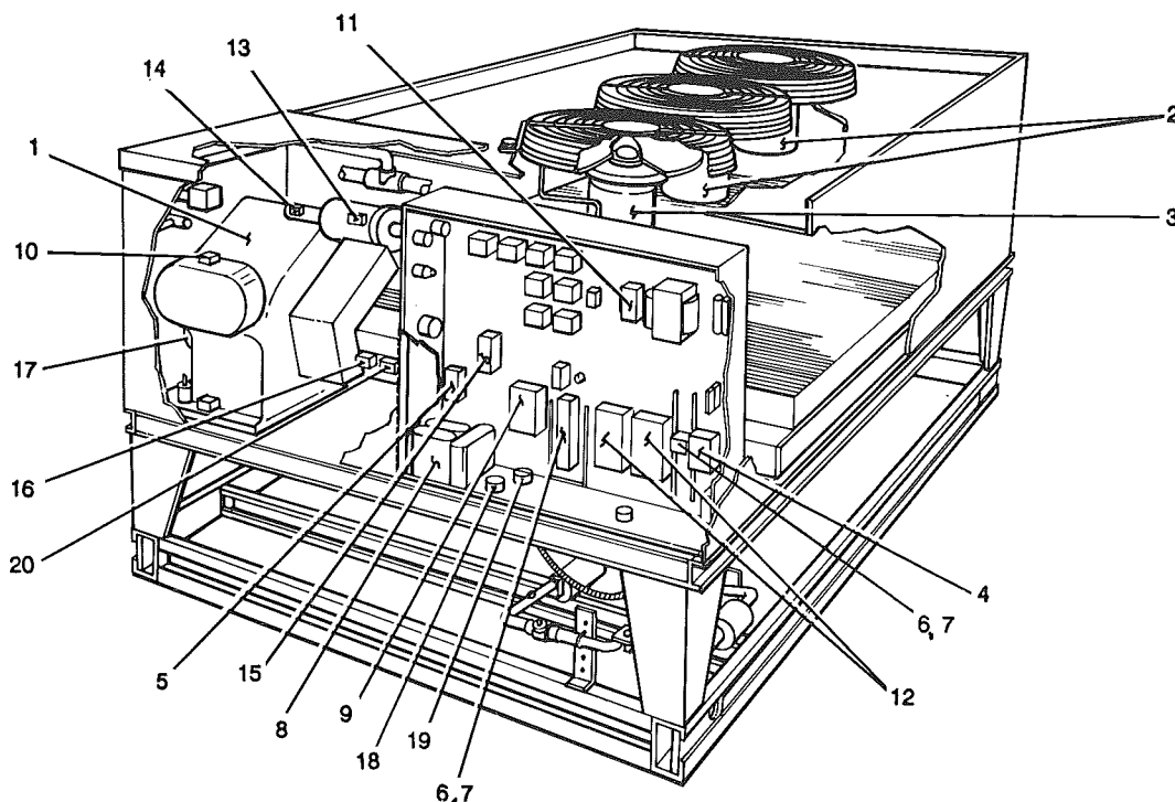
FIG. 1 - AIR COOLED WATER CHILLER
