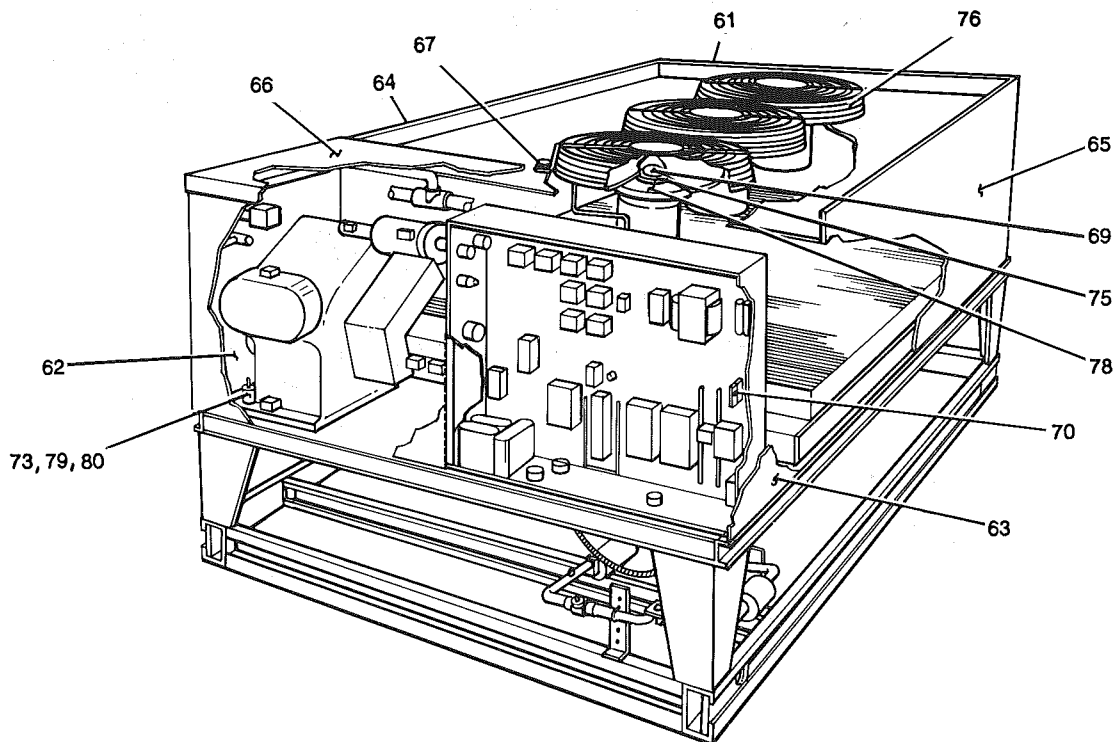
FIG. 4 - AIR COOLED WATER CHILLER
