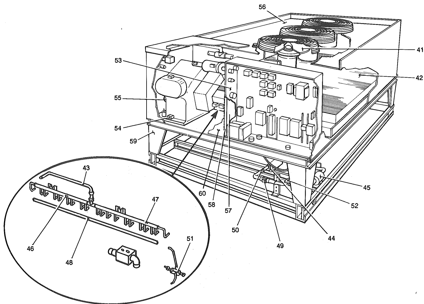
FIG. 3 - AIR COOLED WATER CHILLER
