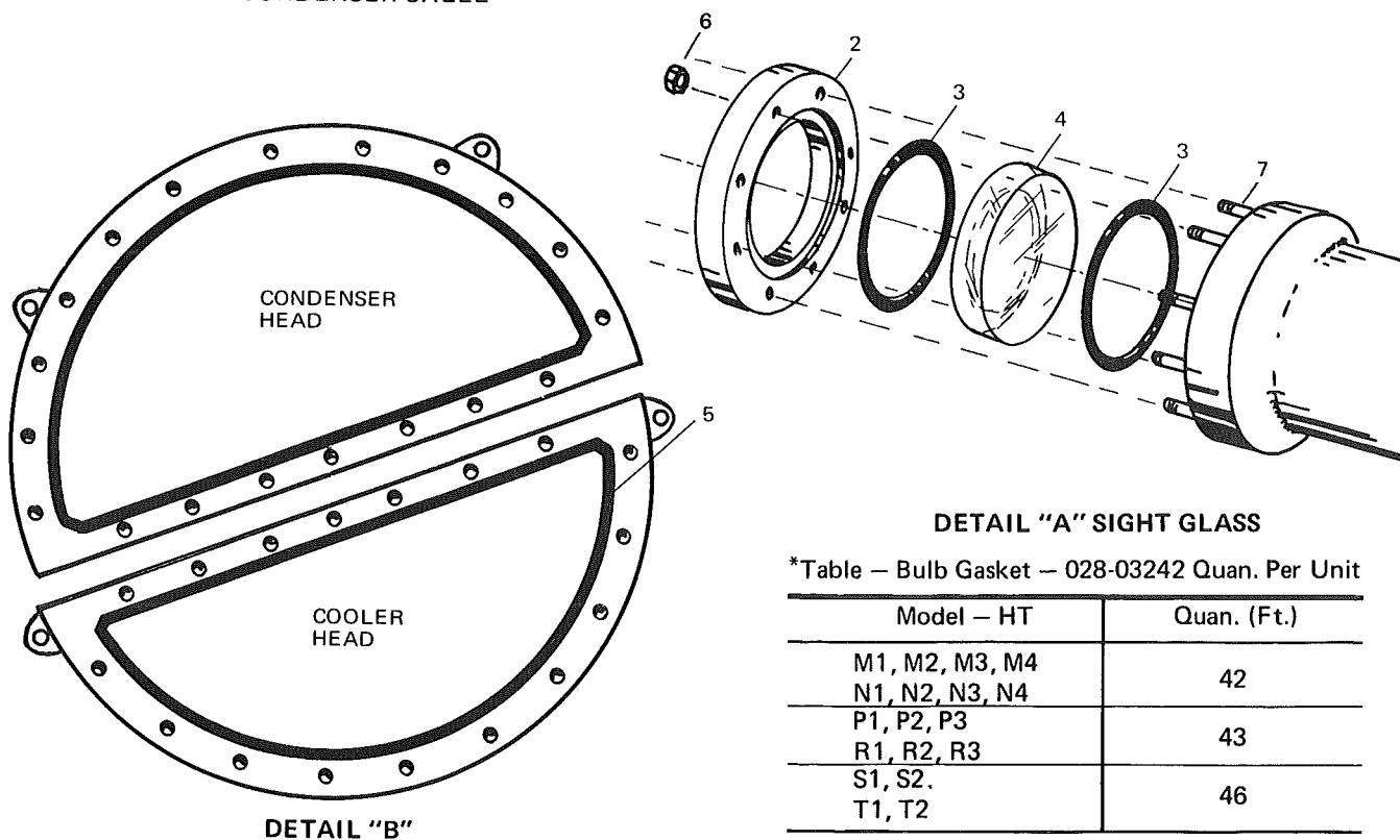
FIG. 1— COOLER—CONDENSER SHELL
