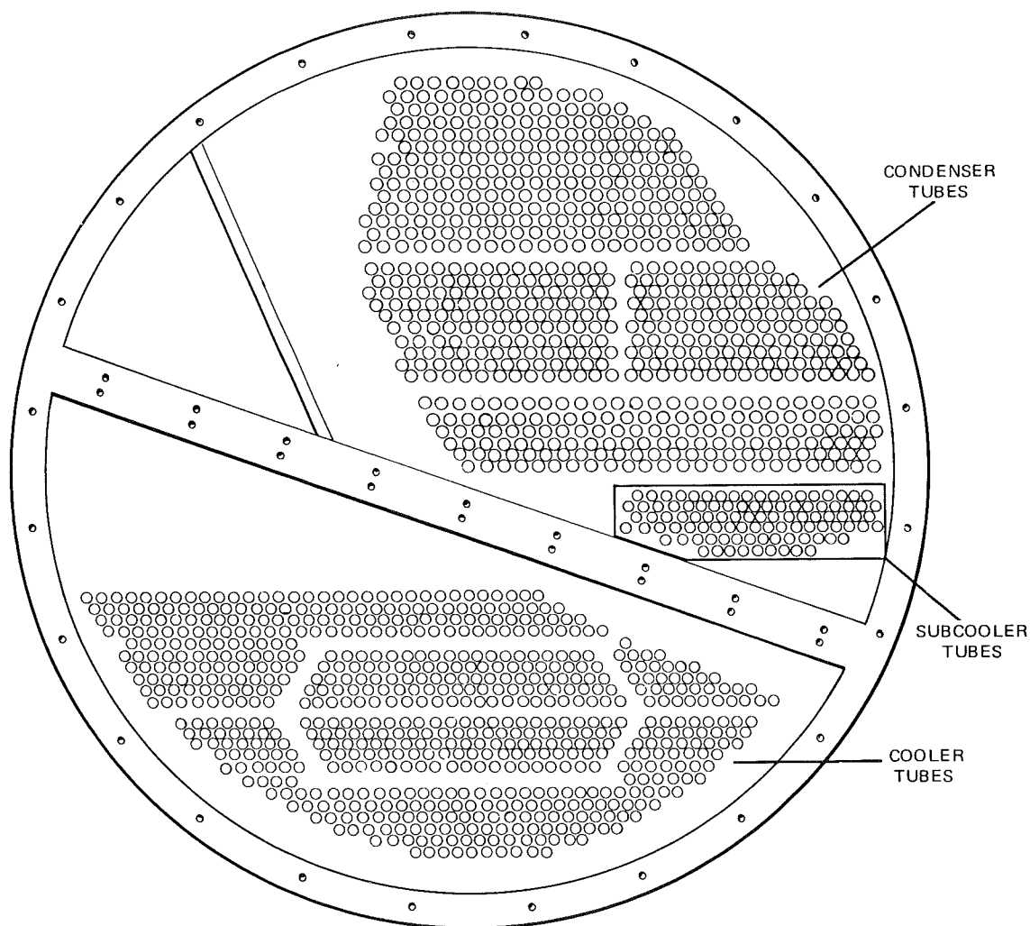
FIG. 3— COOLER AND CONDENSER TUBES—MOTOR END VIEW
