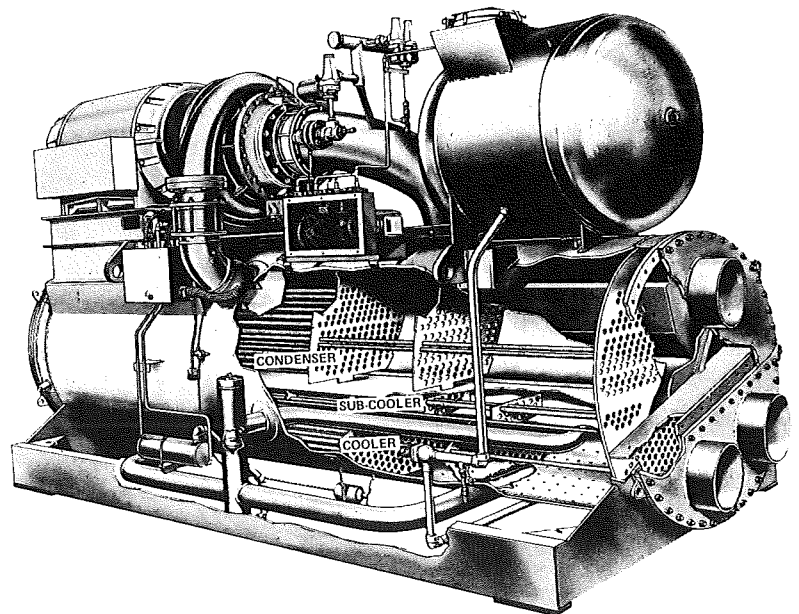
OT TURBOPAK
