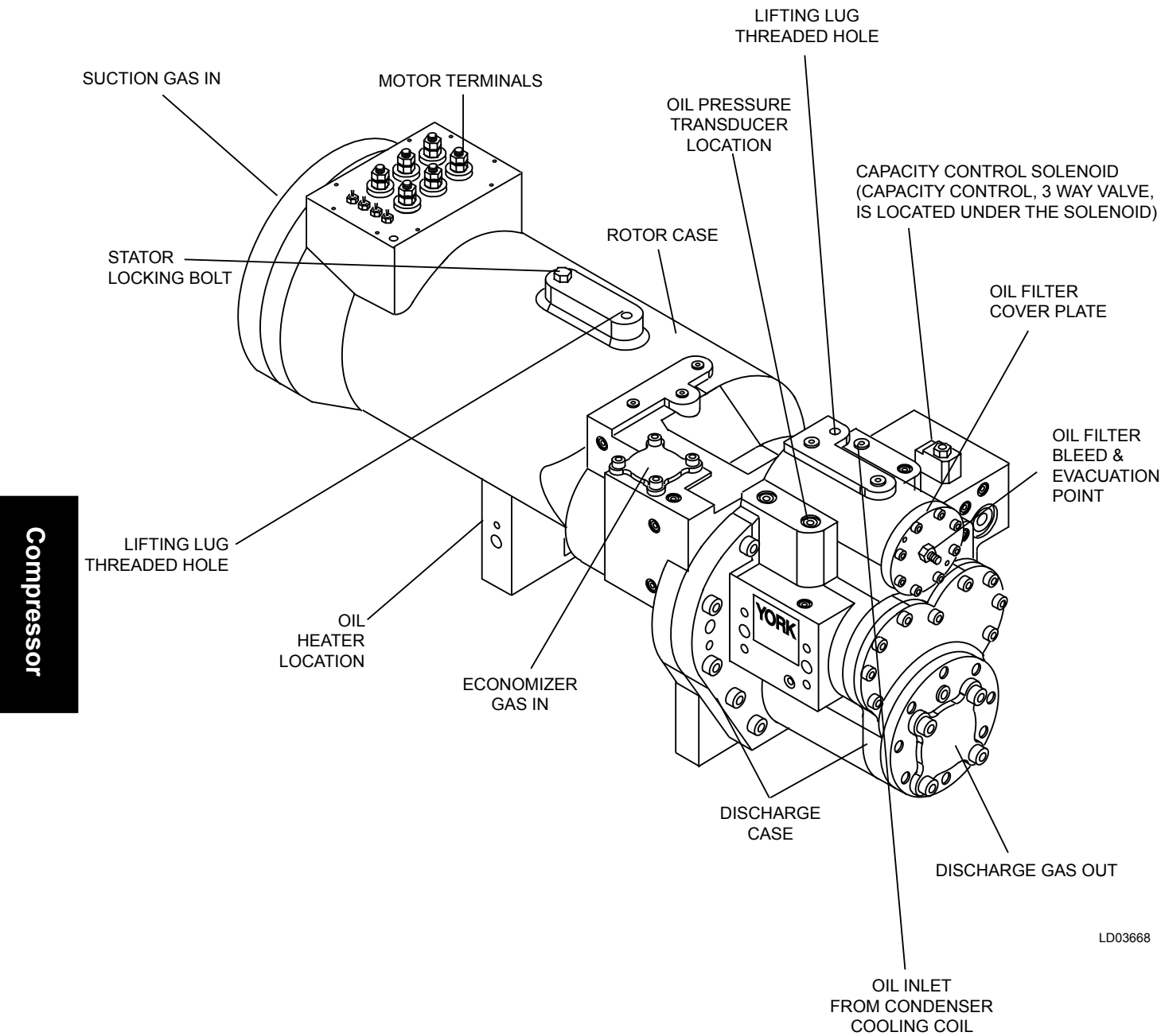
FIG. 11 – DXS COMPRESSOR OUTLINE
