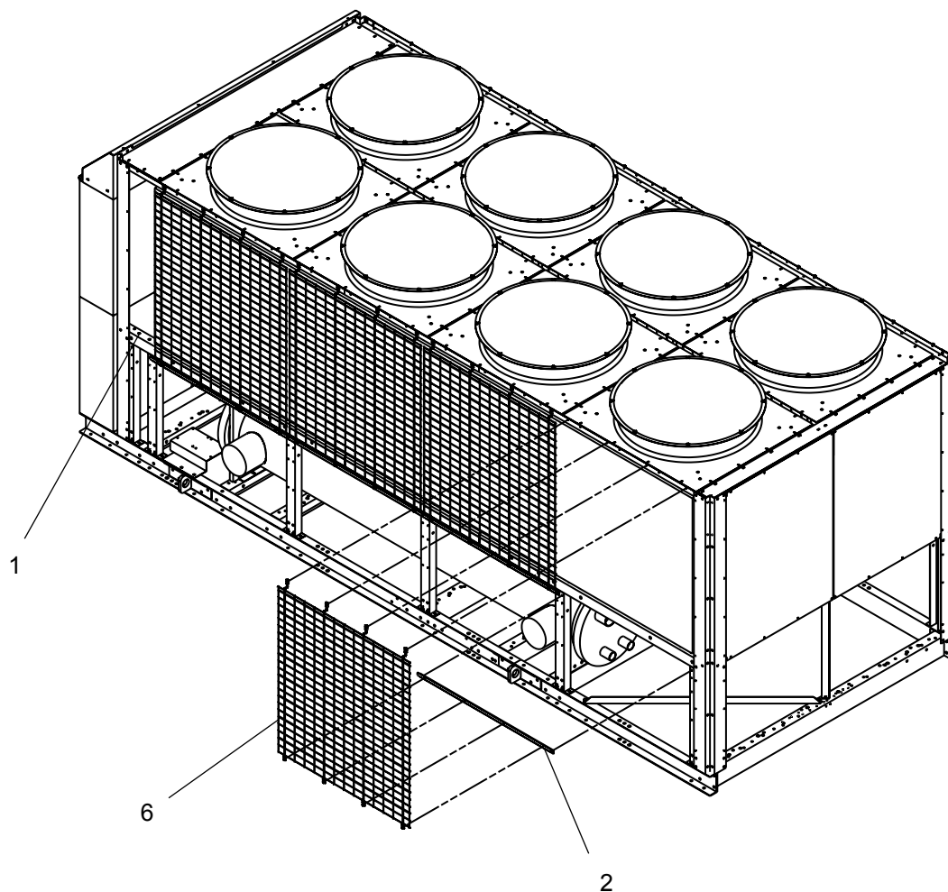
FIG. 29 – WIRE ENCLOSURE - 16'-0" KIT IS SHOWN.
