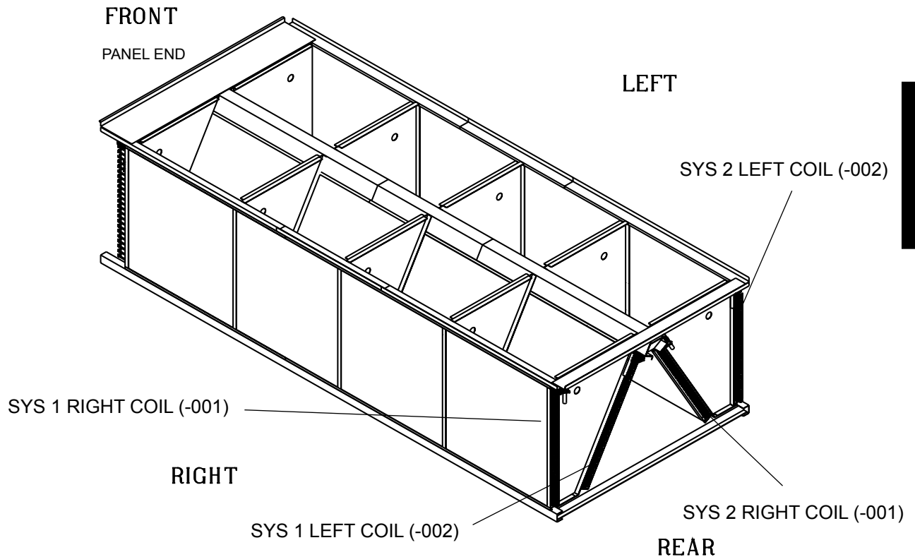
FIG. 3 – CONDENSER COIL LAYOUT - 16'-0" SHOWN
