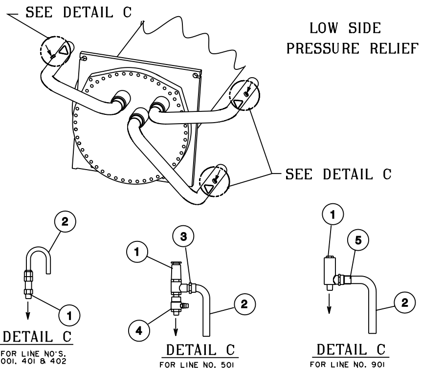
FIG. 10 – RELIEF VALVES AND HP CUTOUT SWITCH (REF. TABLE 7, PAGE 14)
