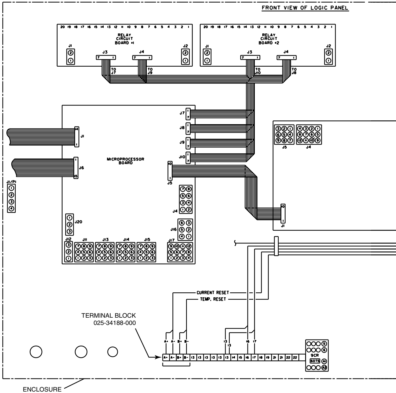
FIG. 33 – REMOTE CURRENT/TEMPERATURE RESET WIRING KIT
