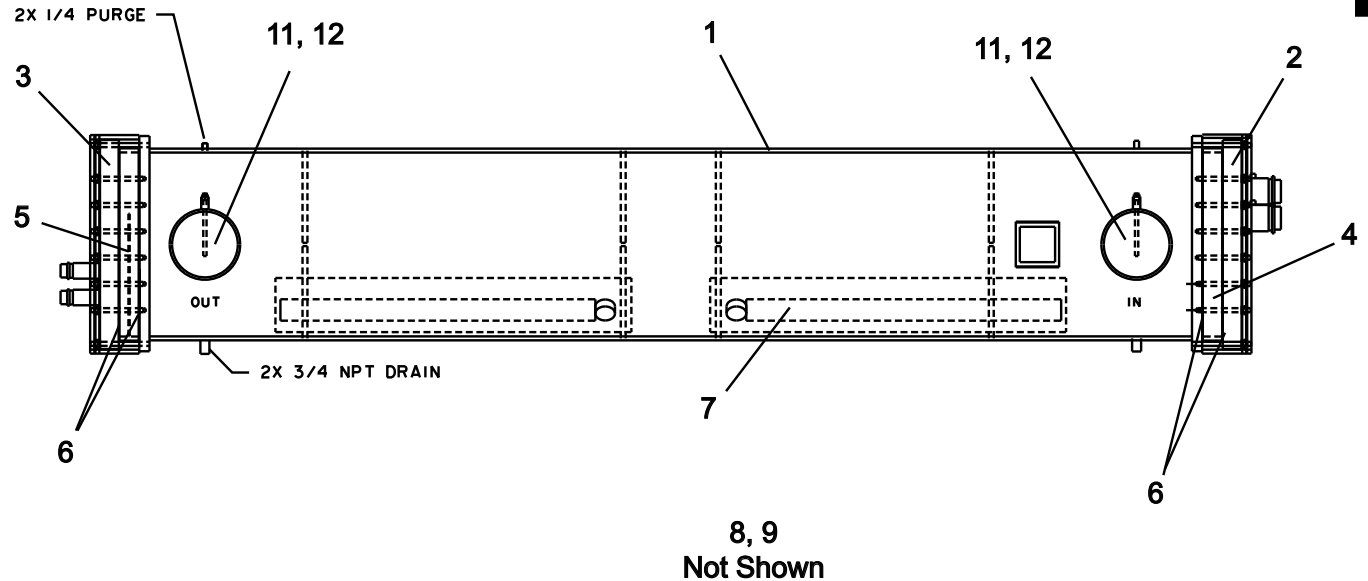
FIG. 1 –EVAPORATOR COMPONENTS
