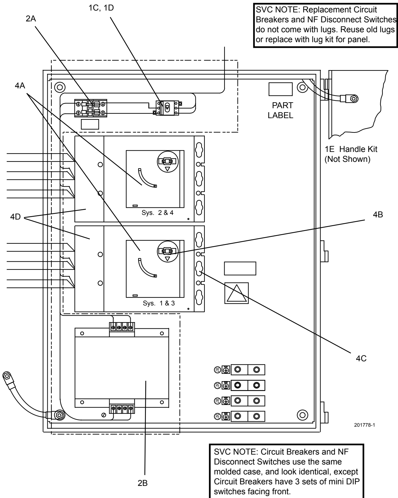
FIG. 27 – OPTION PANEL SHOWN WITH CIRCUIT BREAKER OR NON-FUSED DISCONNECT SWITCH (REF. TABLE 22, PAGES 48 AND 49)
