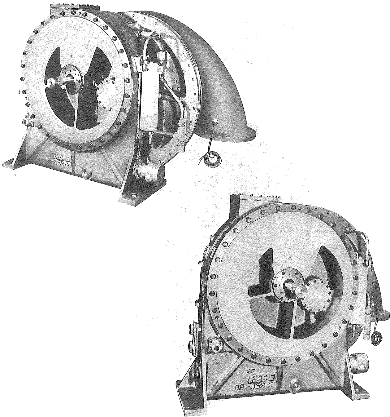
FIG. 1 — OPEN TYPE COMPRESSOR, MODEL LKC
