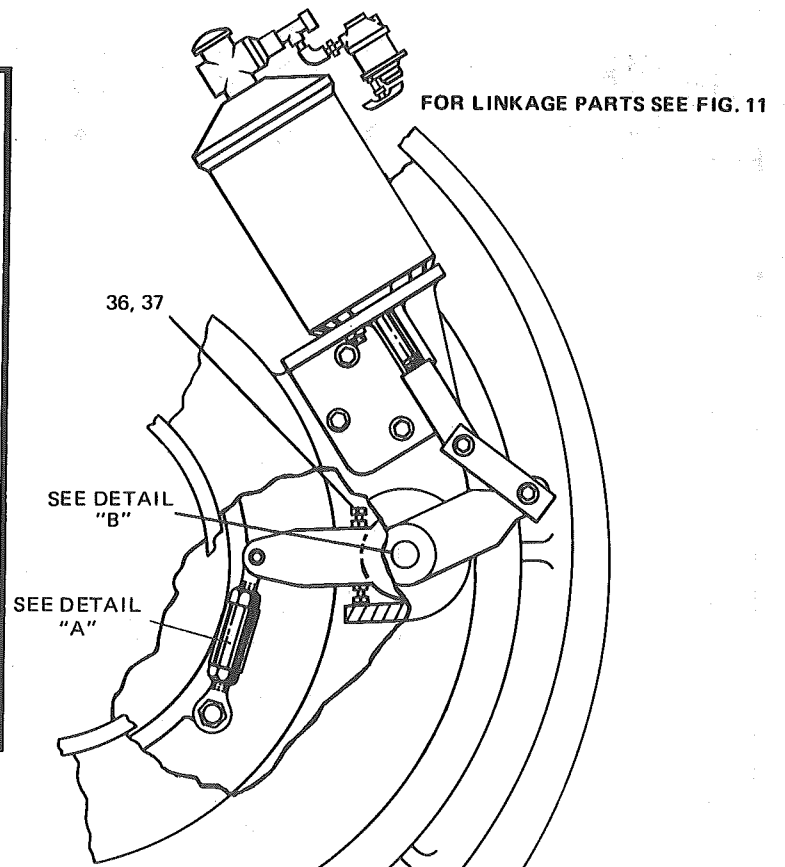
FIG. 5- PNEUMATIC PRV POSITION LEVER - ADJUSTMENT PARTS
