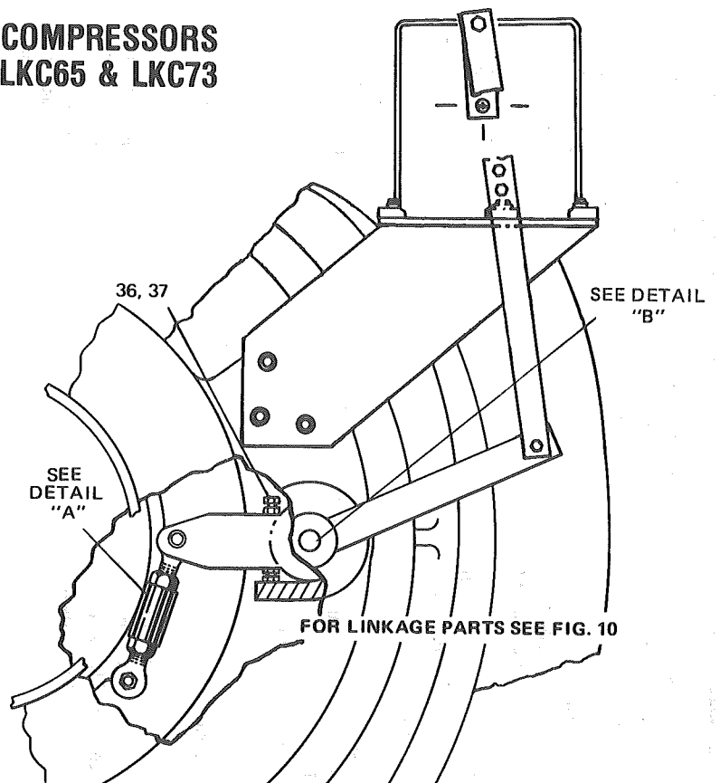
FIG. 4- ELECTRIC MOTOR LEVER - ADJUSTMENT PARTS
