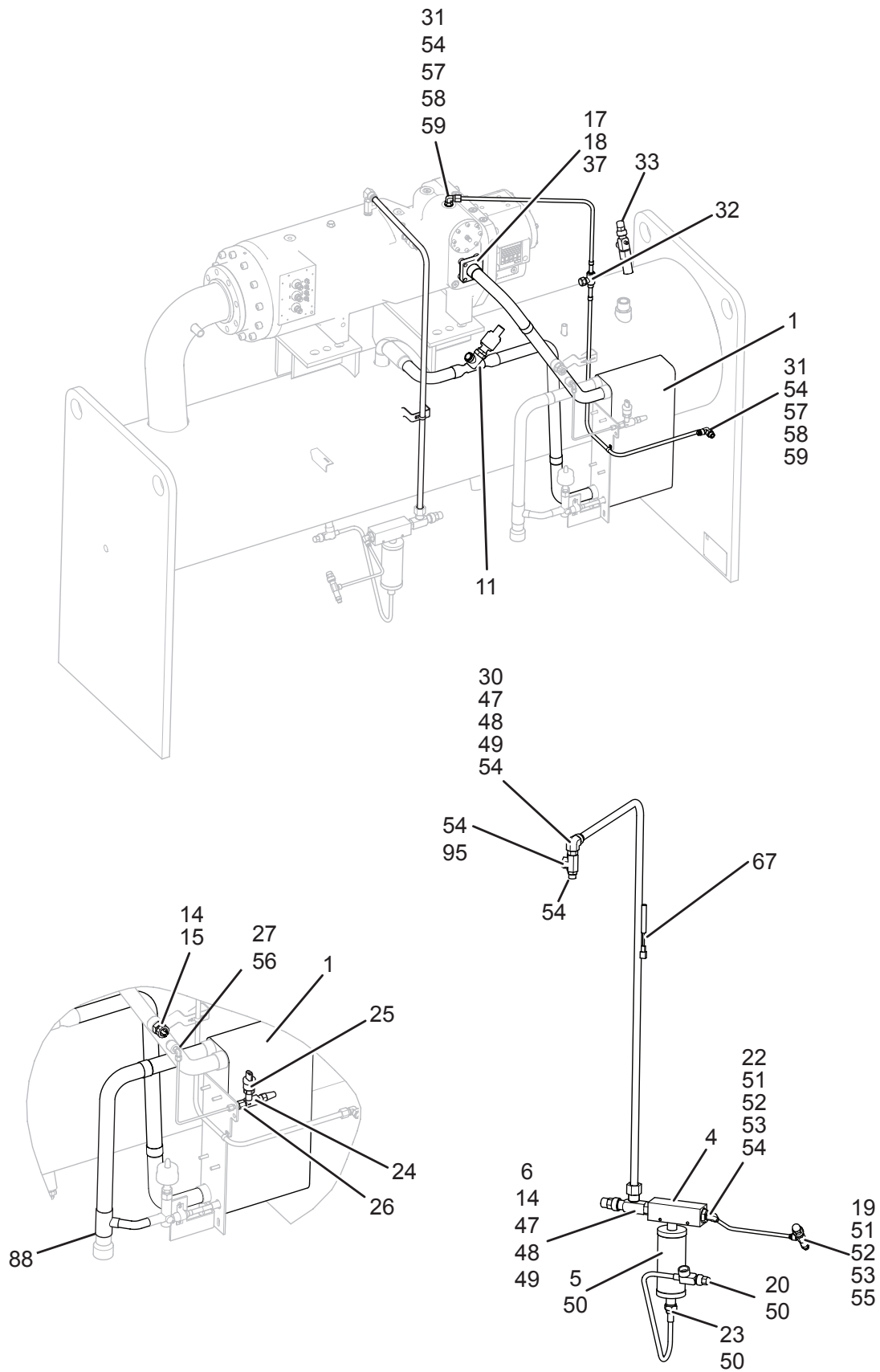
FIGURE 7 - UNIT PIPING FOR SINGLE SYSTEM
