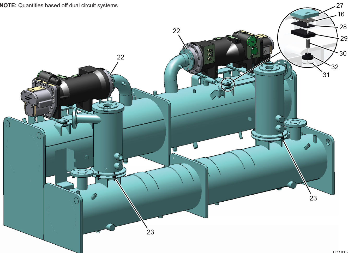
FIGURE 1 - UNIT COMPONENTS
