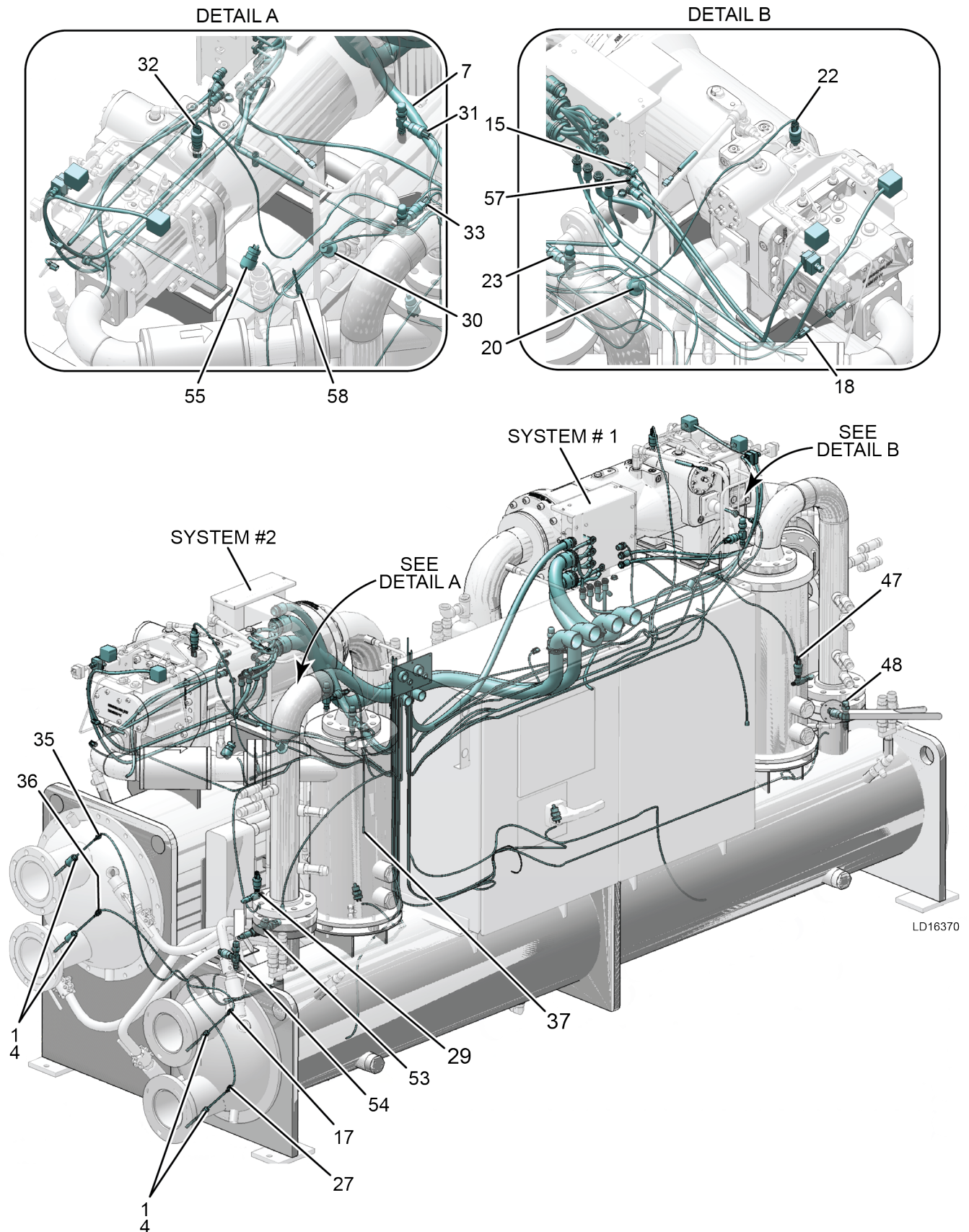
FIGURE 55 - SYSTEM WIRING
