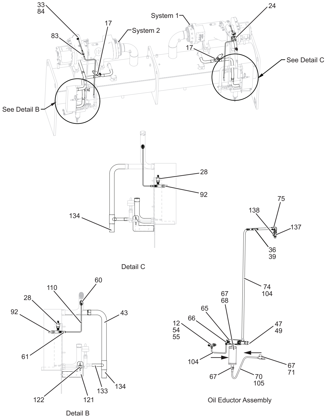
FIGURE 9 - UNIT PIPING FOR DUAL SYSTEMS
