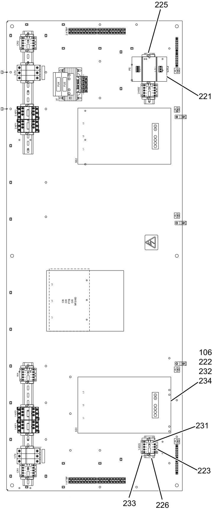
FIGURE 22 - POWER/CONTROL ASSEMBLY (SOFT STARTER)
