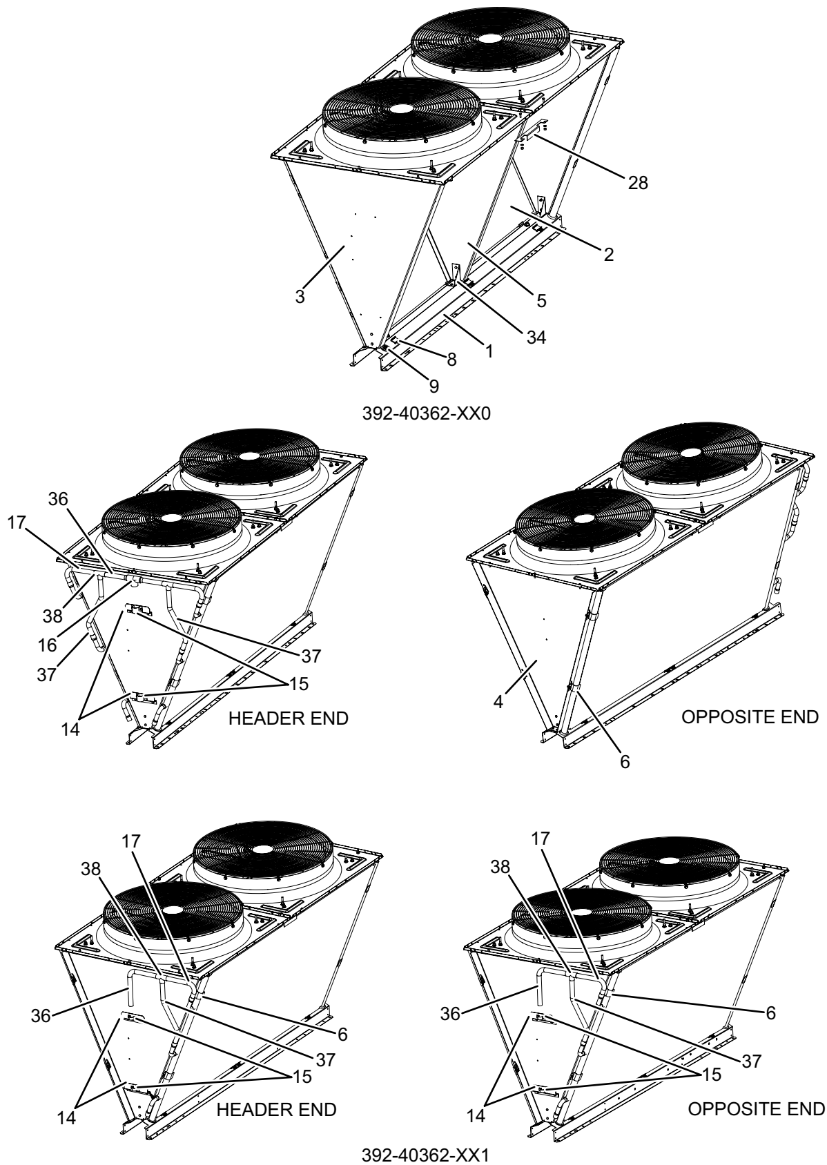
FIGURE 8 - CONDENSER COILS
