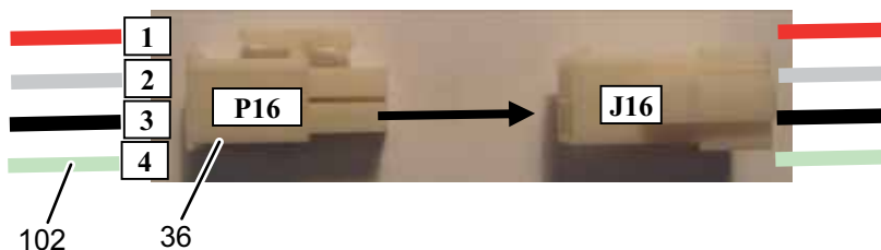
FIGURE 15 - SYSTEM WIRING
