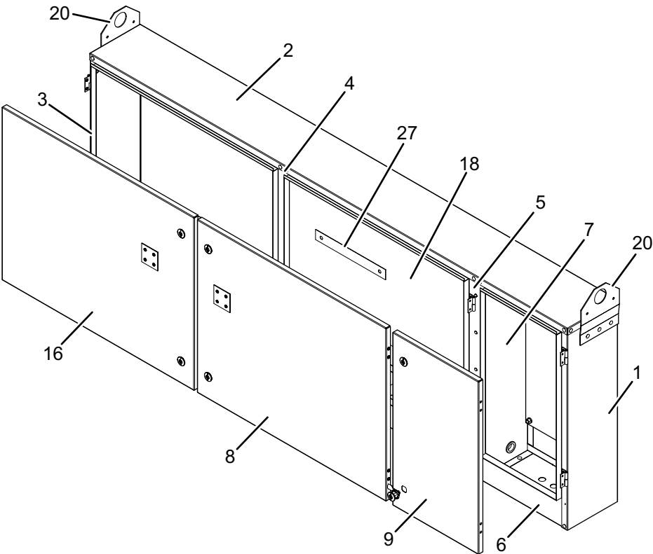
FIGURE 25 - POWER ENCLOSURE
