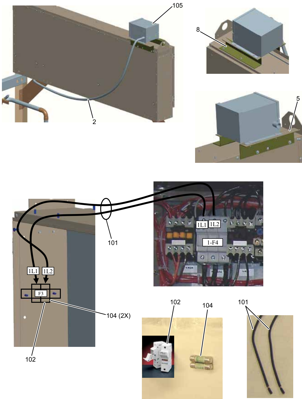
FIGURE 27 - CONTROL TRANSFORMER
