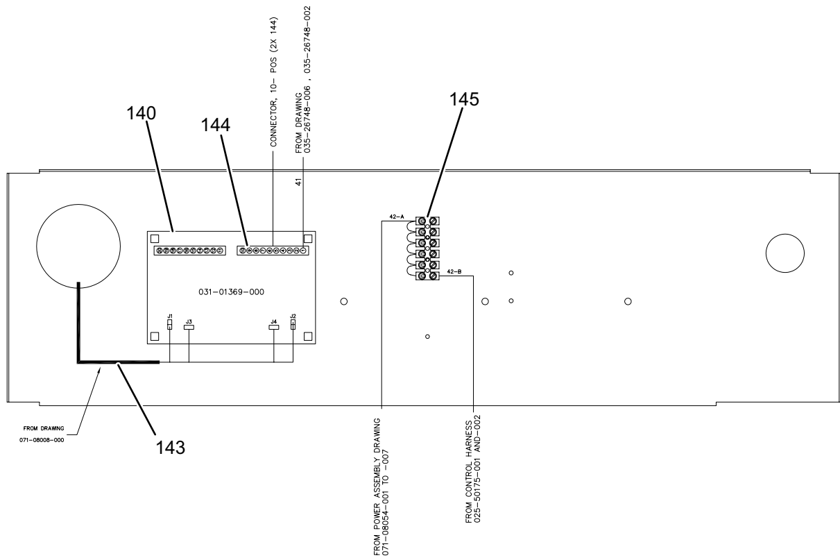
FIGURE 17 - SOLENOID ASSEMBLY
