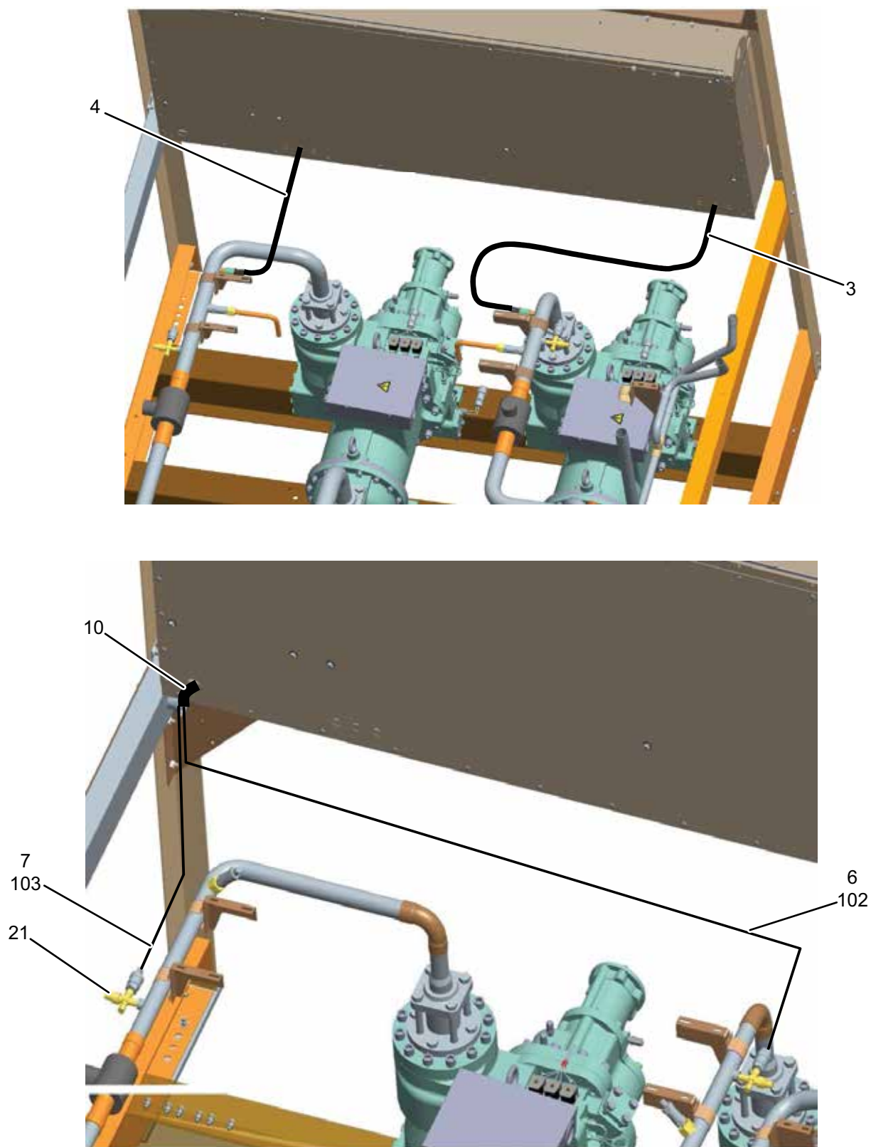
FIGURE 12 - SYSTEM WIRING
