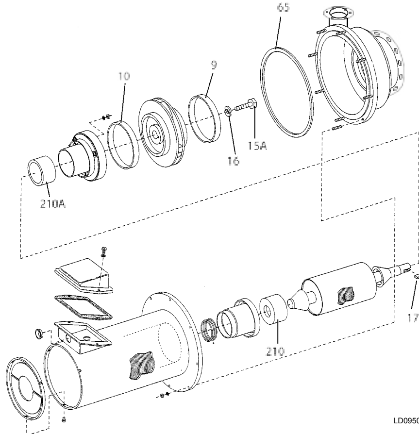
FIG. 5 – Exploded View of Pump, All Pump Styles.
