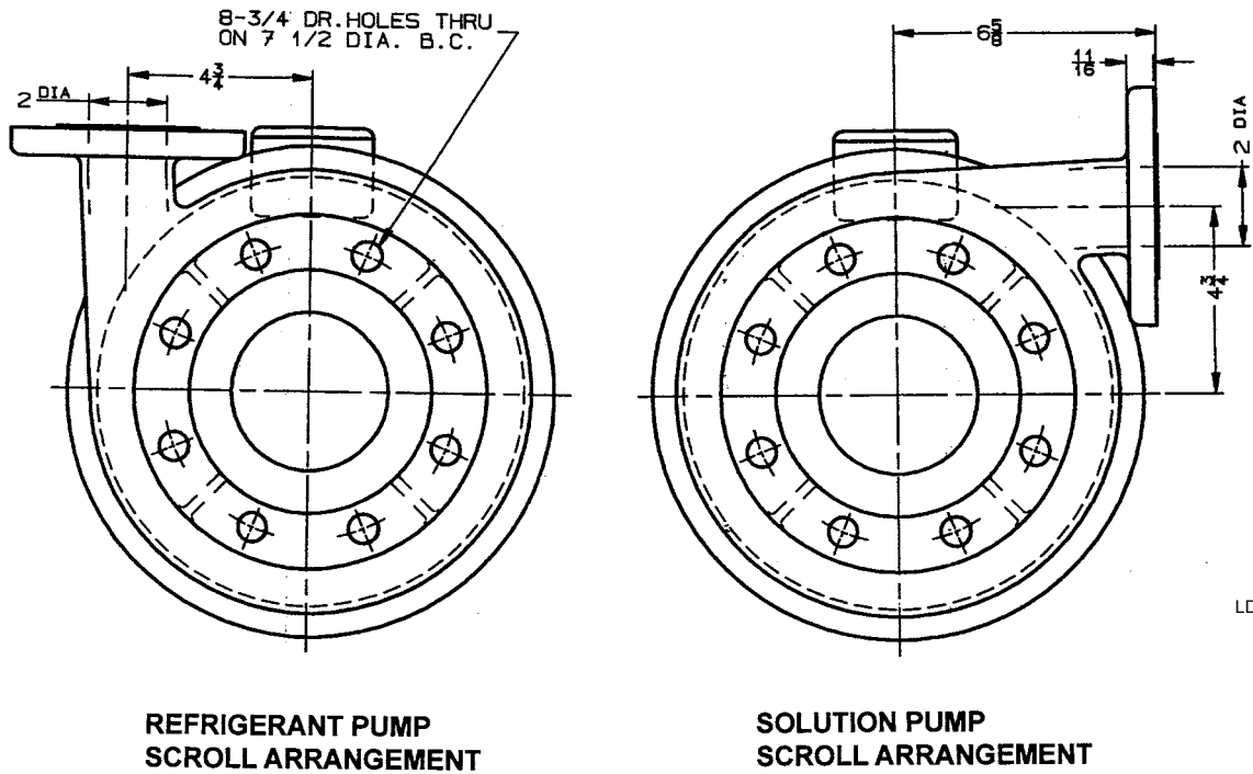
FIG. 7 – Pump Style "A" Dimensions
