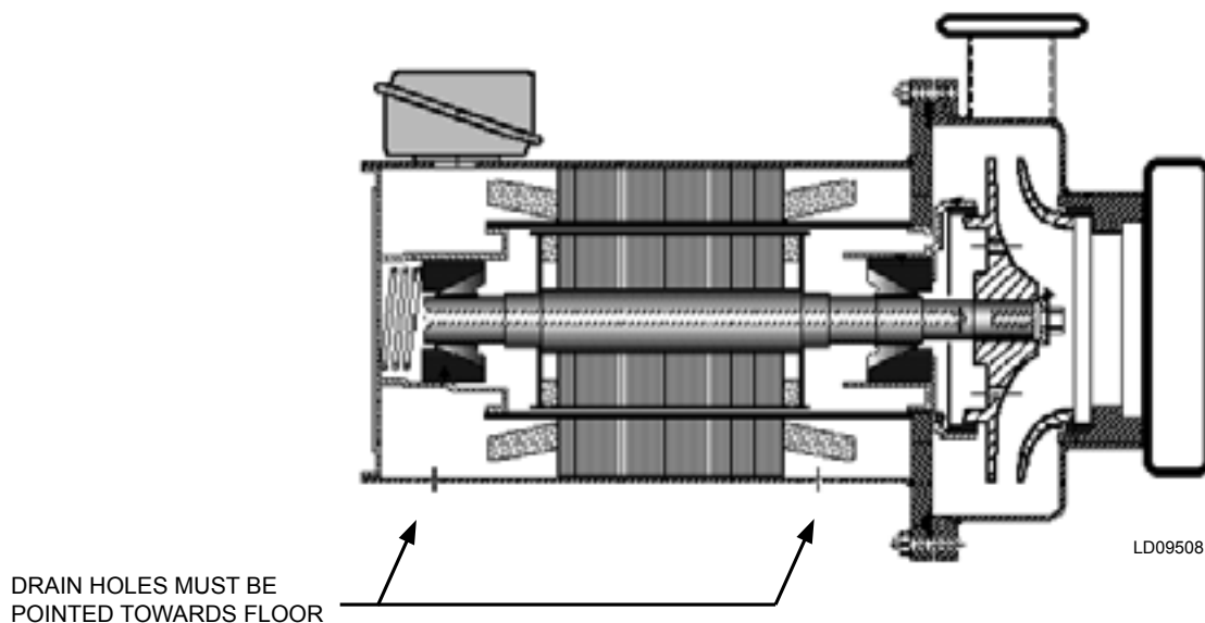
FIG. 6 – View of Pump Cross Section
