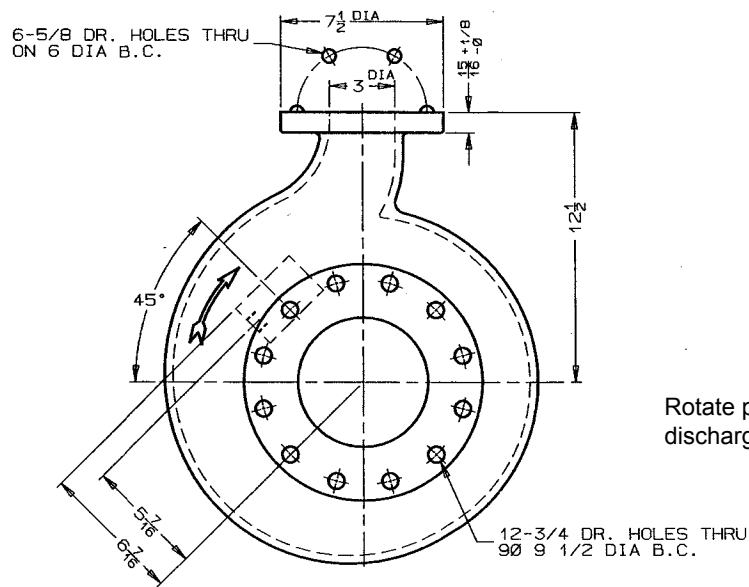
FIG. 8 – Pump Style "B" Dimensions
