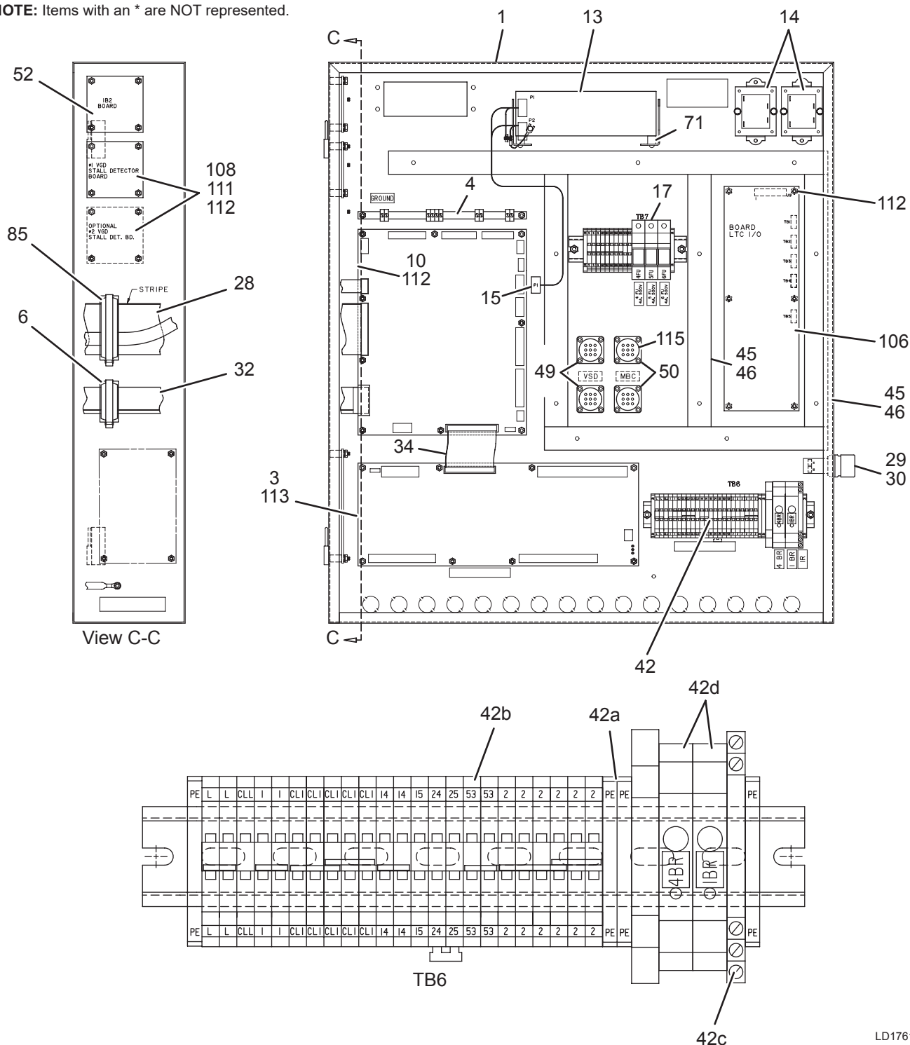
FIGURE 18 - OPTIVIEW CONTROL PANEL
