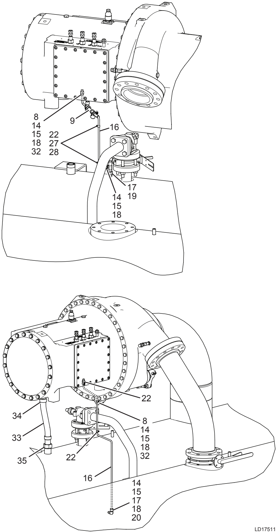
FIGURE 16 - SYSTEM PIPING
