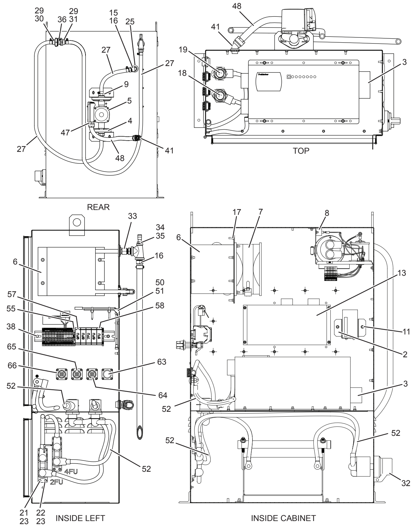
FIGURE 23 - POWER PANEL
