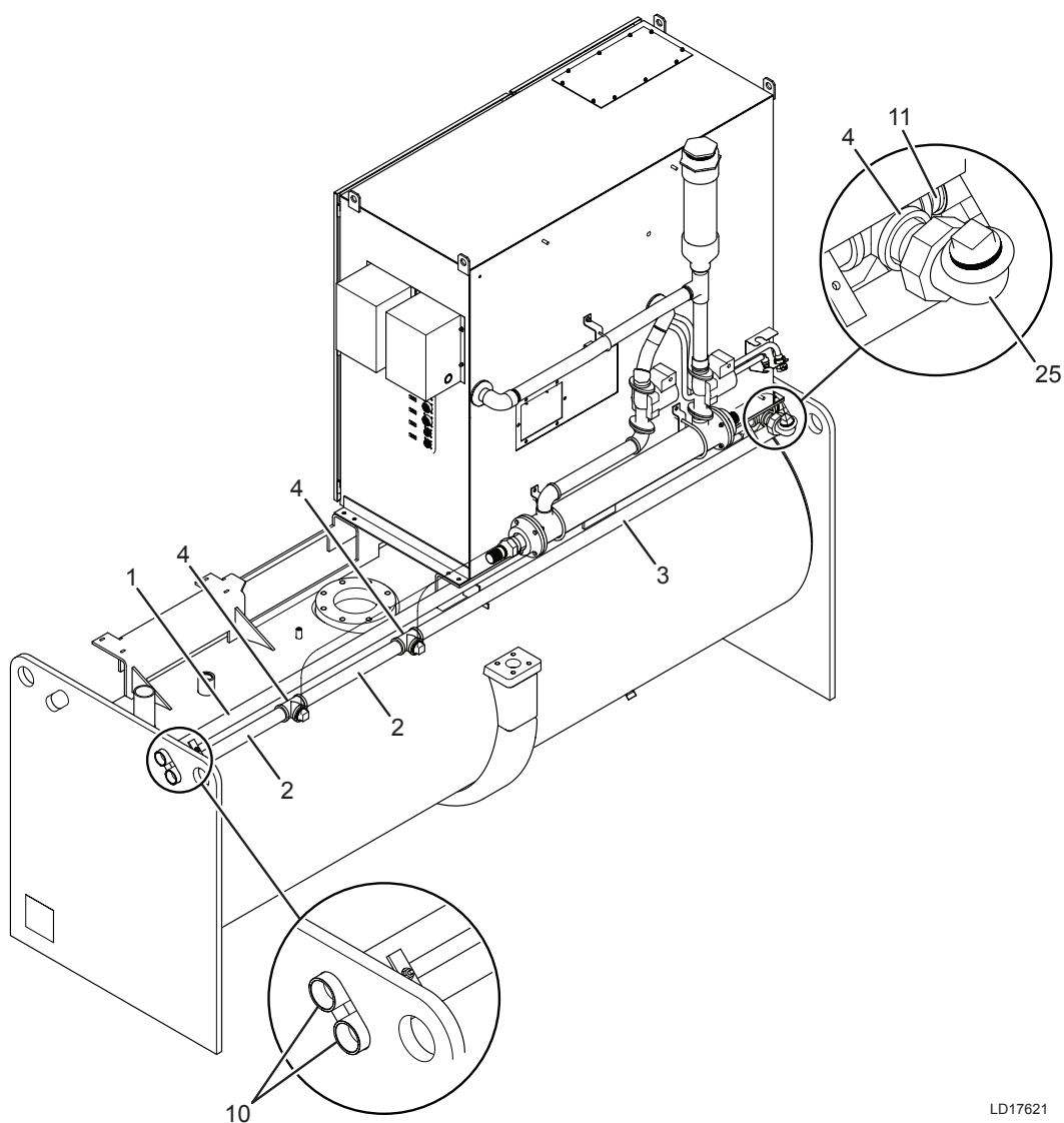
FIGURE 26 - VSD WATER PIPING
