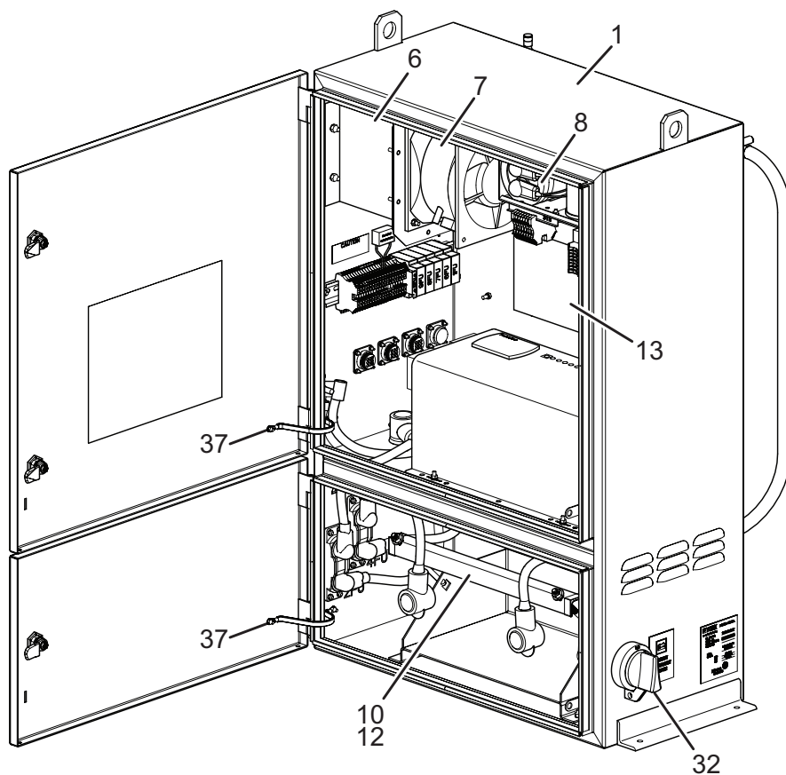
FIGURE 22 - POWER PANEL
