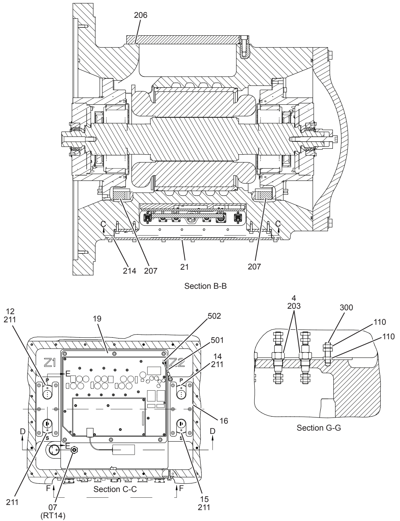
FIGURE 10 - MOTOR COMPONENTS
