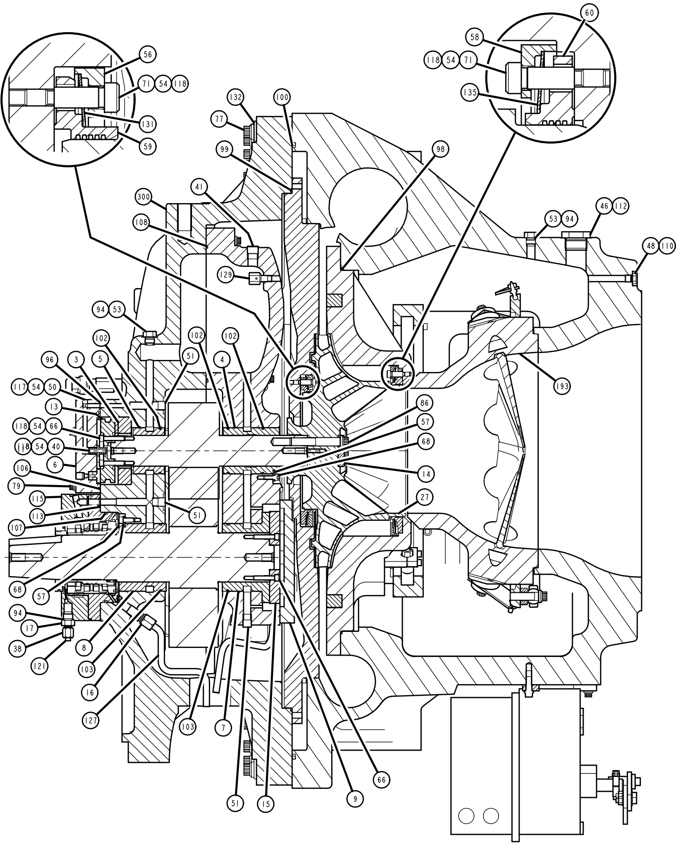
FIG. 1 – K1 COMPRESSOR
