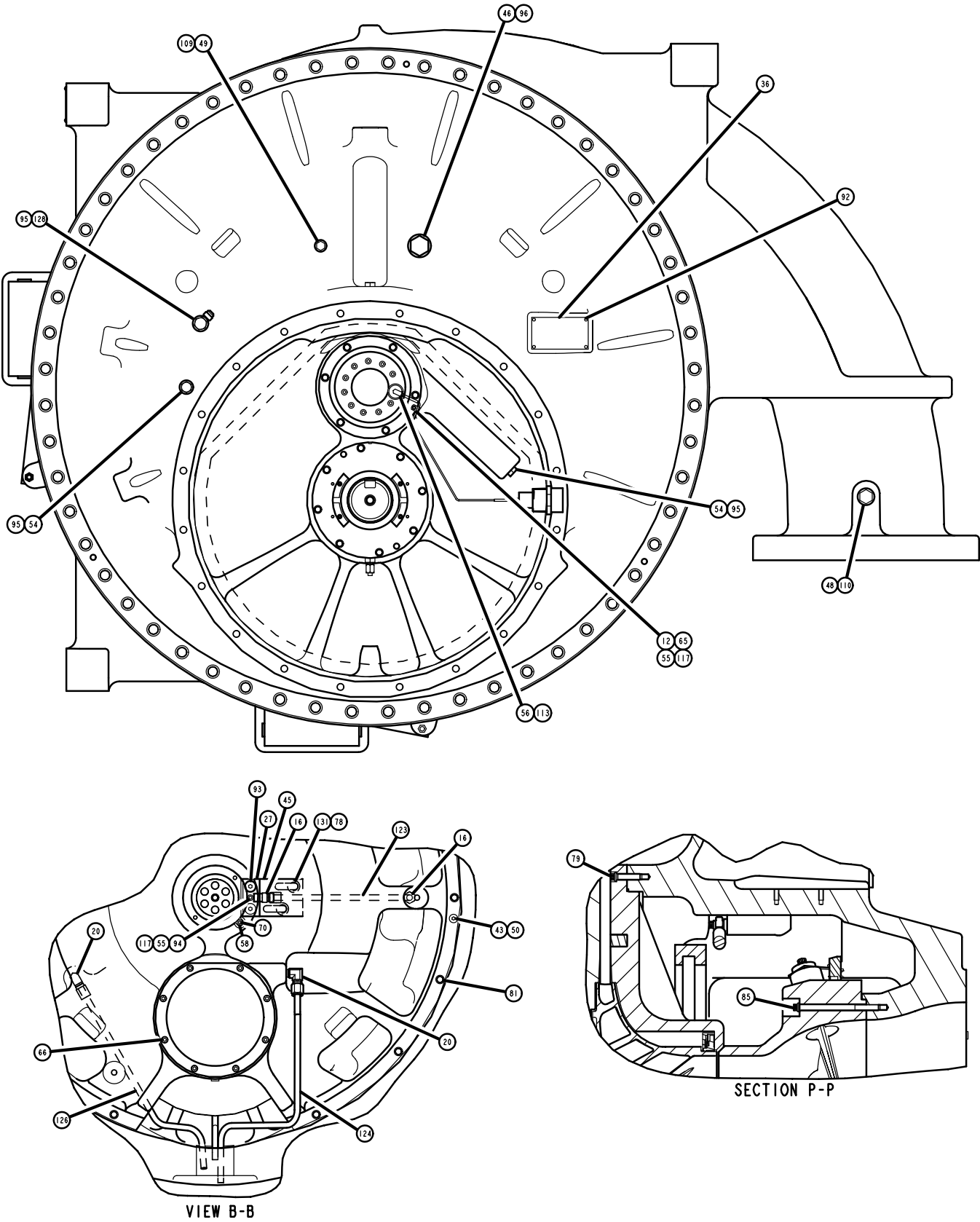
FIG. 20 – K4 COMPRESSOR
