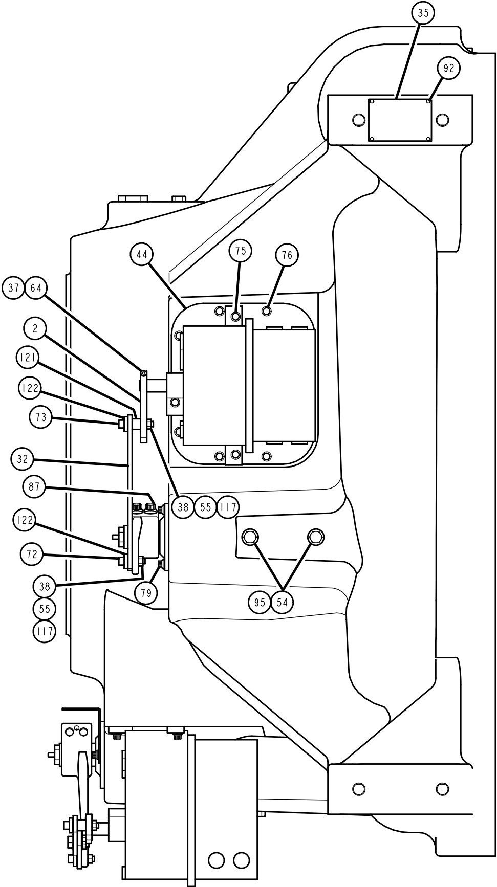
FIG. 22 – K4 COMPRESSOR
