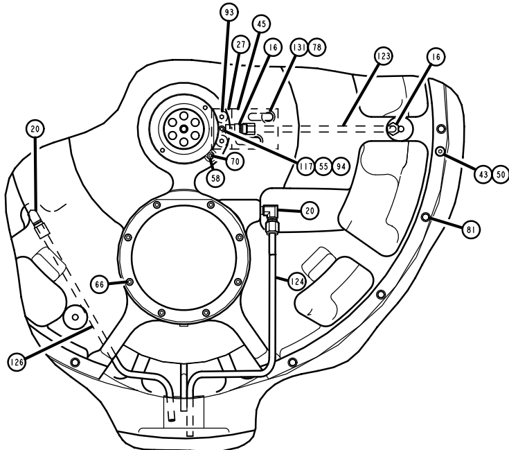
VIEW B-B
