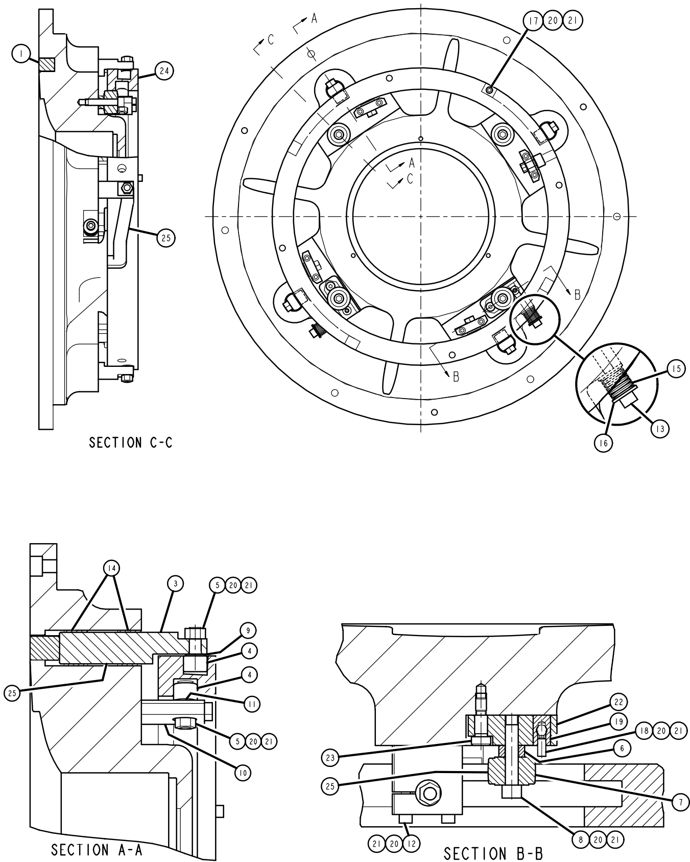
FIG. 12 – VARIABLE GEOMETRY DIFFUSER (K2)
