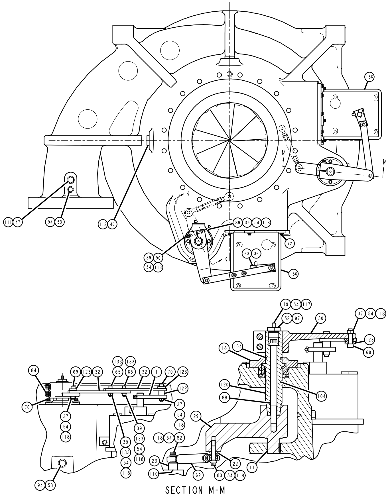
FIG. 3 – K1 COMPRESSOR
