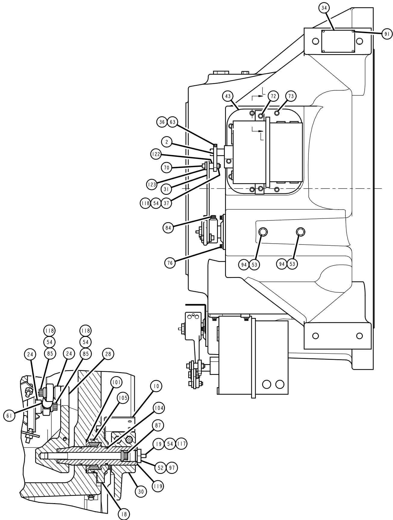
SECTION K-K
