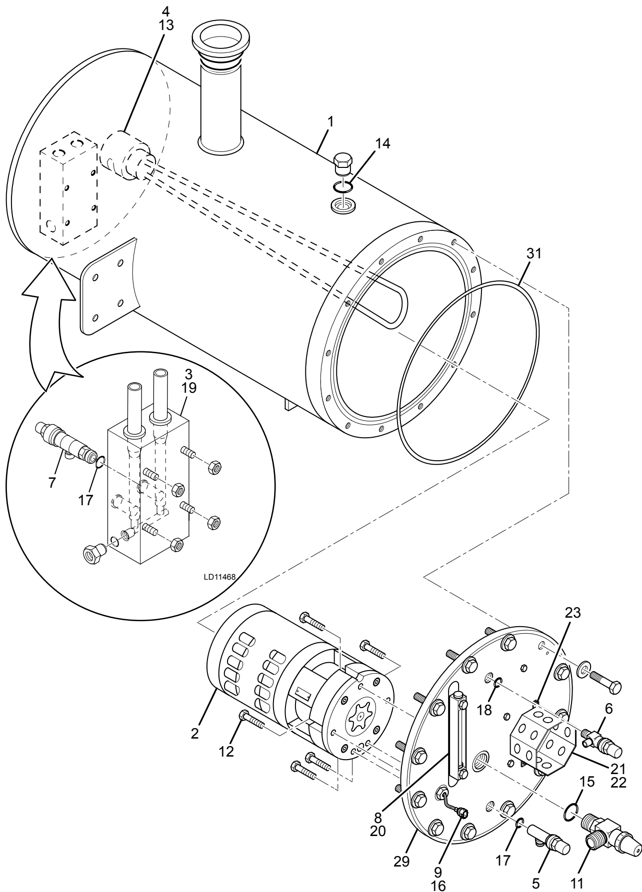
FIG. 25 – OIL PUMP HOUSING ASSEMBLY
