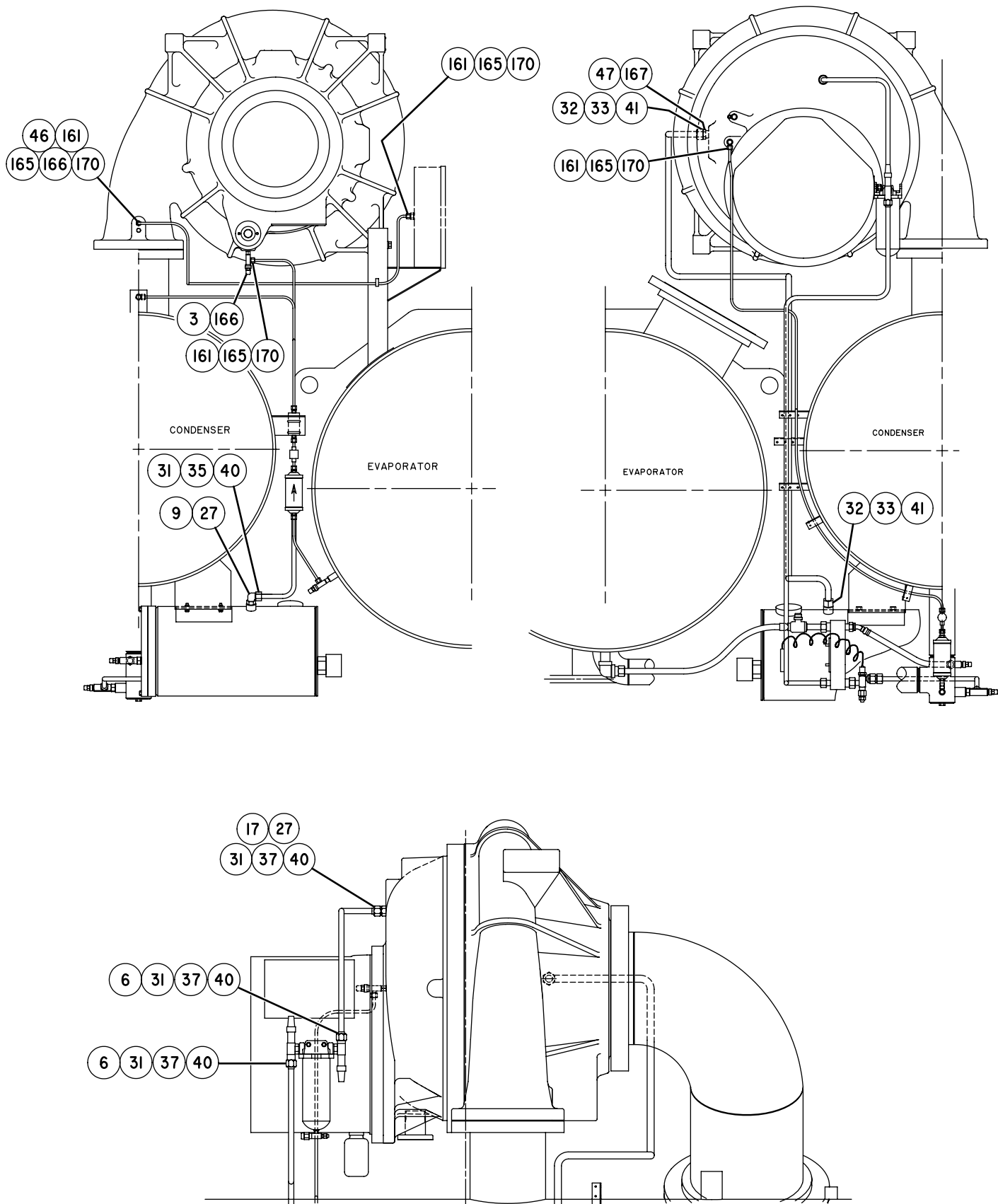
FIG. 27 - COMPRESSOR PIPING
