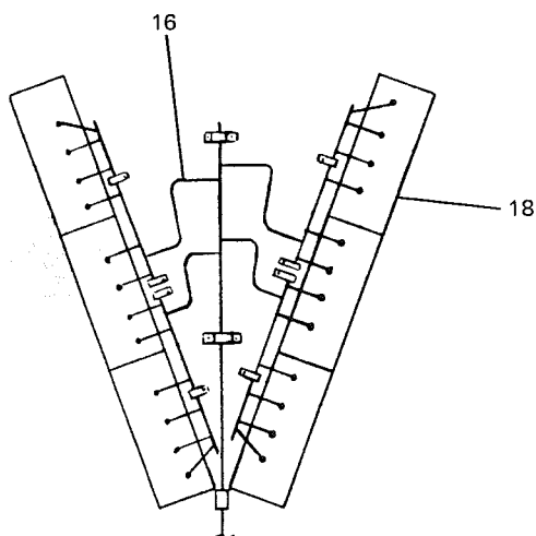
TYPICAL 4 ROW COIL CONFIGURATION
