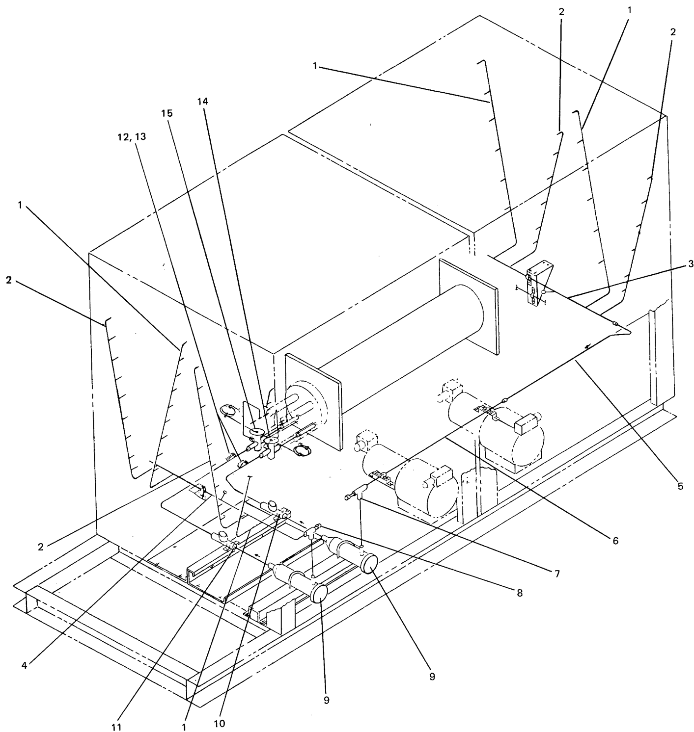
FIG. 17 — REFRIGERANT PIPING COMPONENTS
