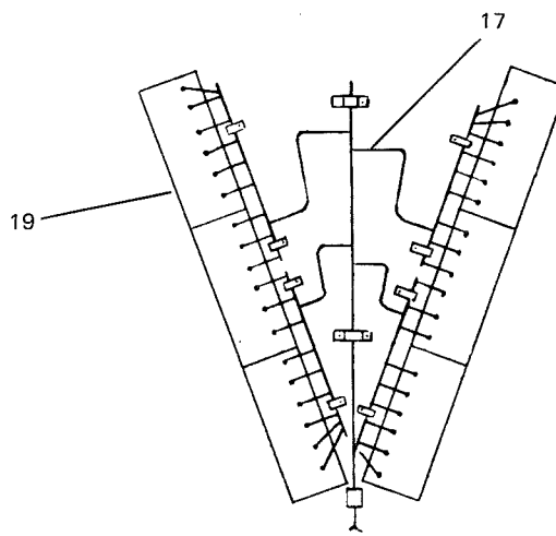
TYPICAL 6 ROW COIL CONFIGURATION
