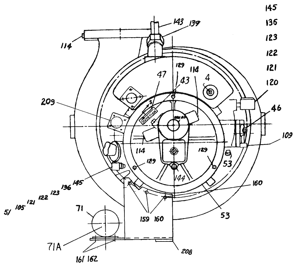
FIG. 2—Front View Compressor
