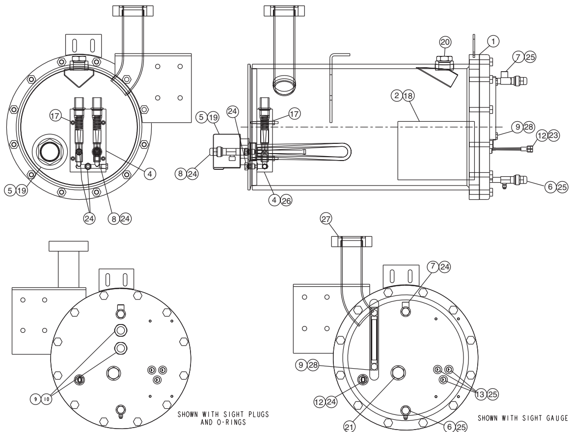
FIG. 8 – HE OIL SUMP
