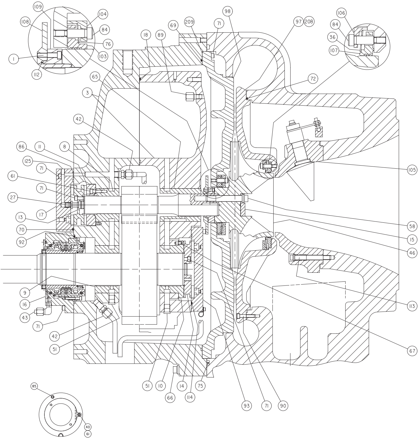
Low Speed Shaft Bearing Retainer
