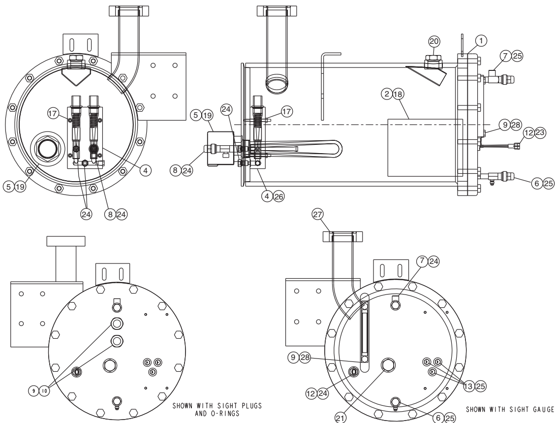
FIG. 25 – HF OIL SUMP
