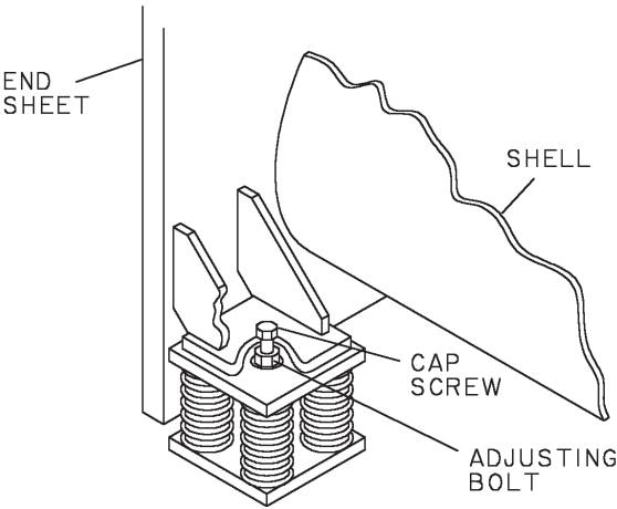
SPRING ISOLATORS
