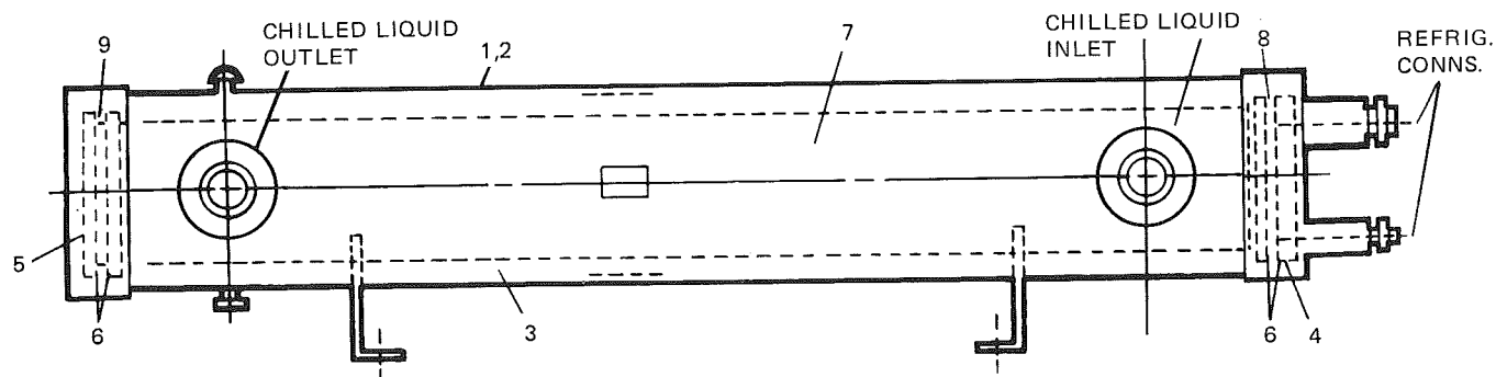
COOLER – YCHA60, 70
