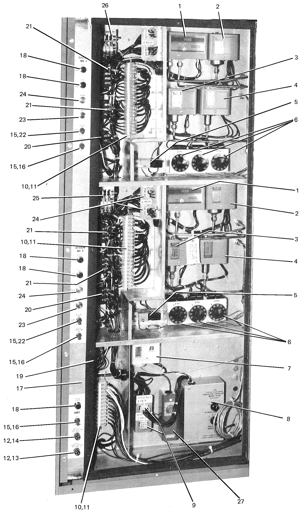
CONTROL PANEL COMPONENTS – YCHA60 & YCHA70
