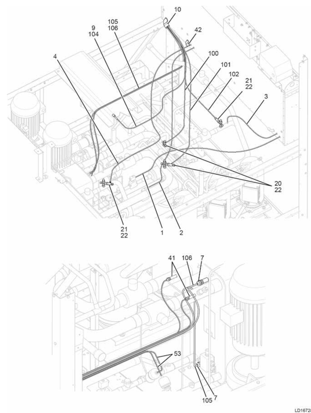
FIGURE 11 - SYSTEM WIRING
