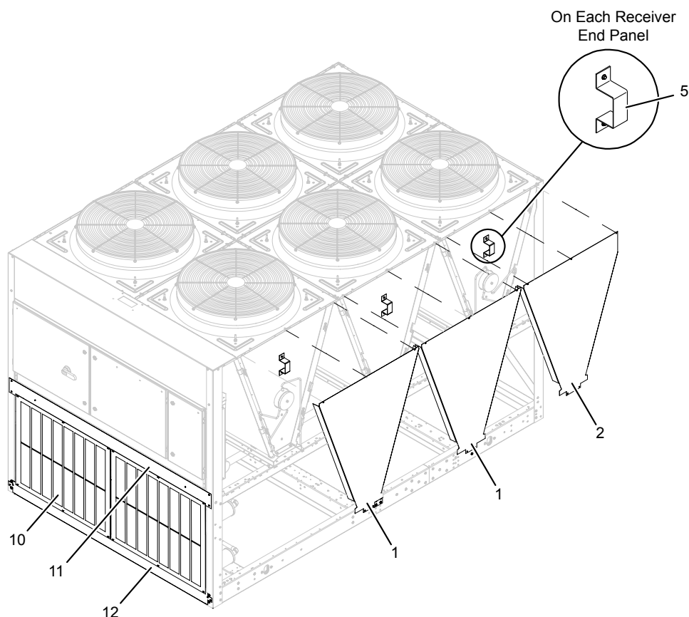
FIGURE 26 - AESTHETIC PANEL
