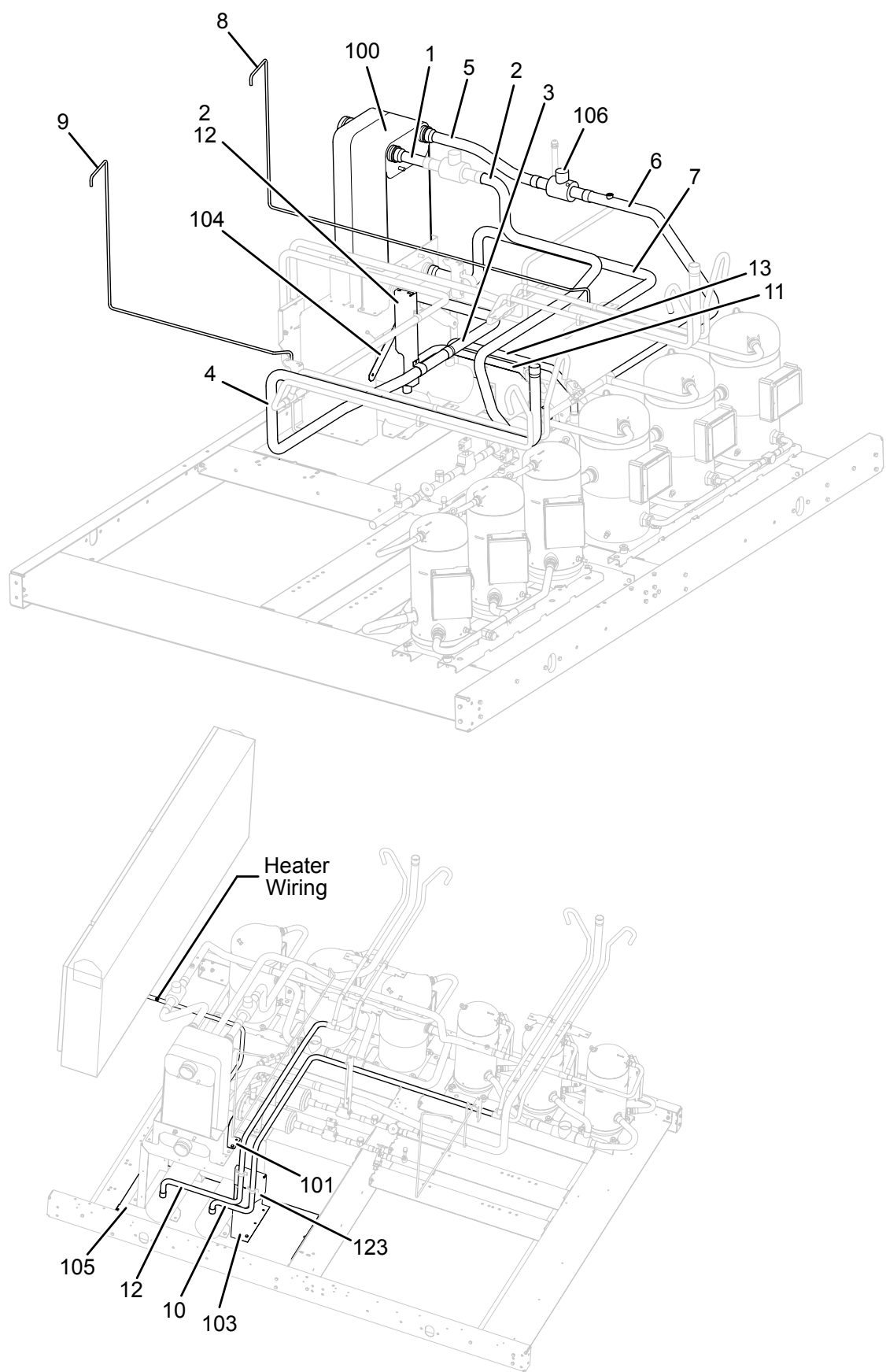
FIGURE 23 - HEAT RECOVERY ASSEMBLY (YLAA0070 - YLAA0090)
