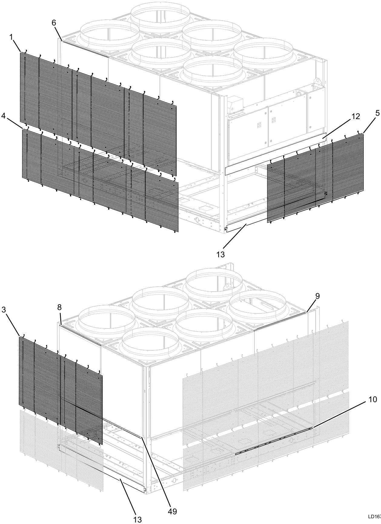
FIGURE 25 - WIRE ENCLOSURE PANELS (YLAA0091 - YLAA0120)
