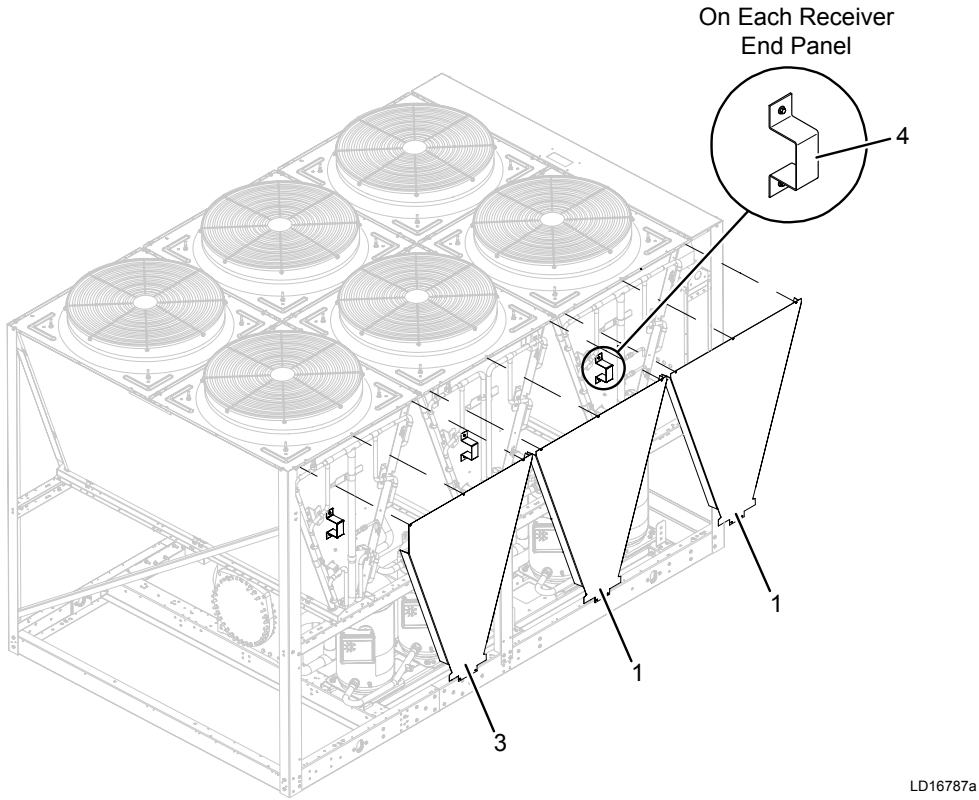
FIGURE 28 - AESTHETIC PANEL (CONT'D)
