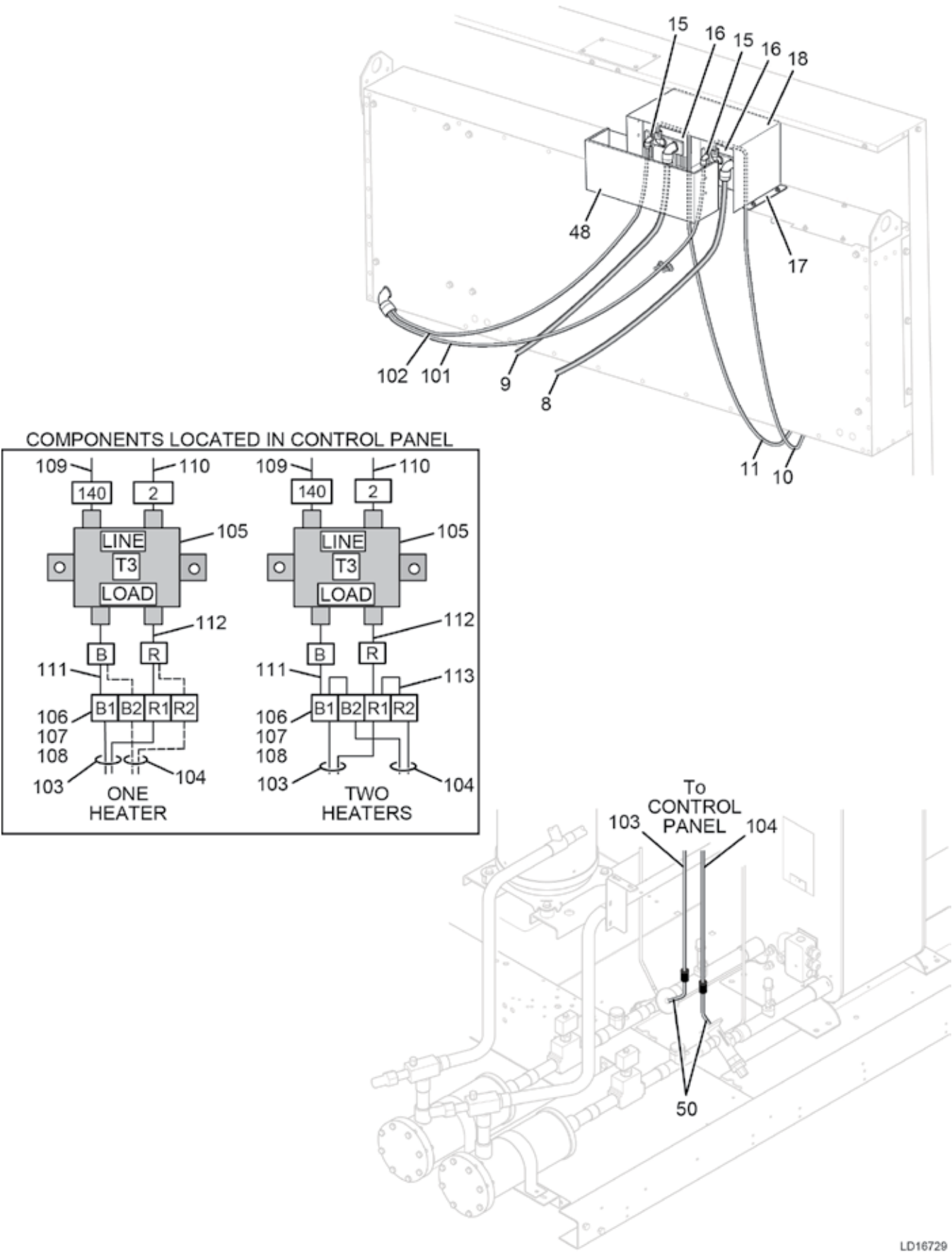
FIGURE 20 - LOW AMBIENT KIT
