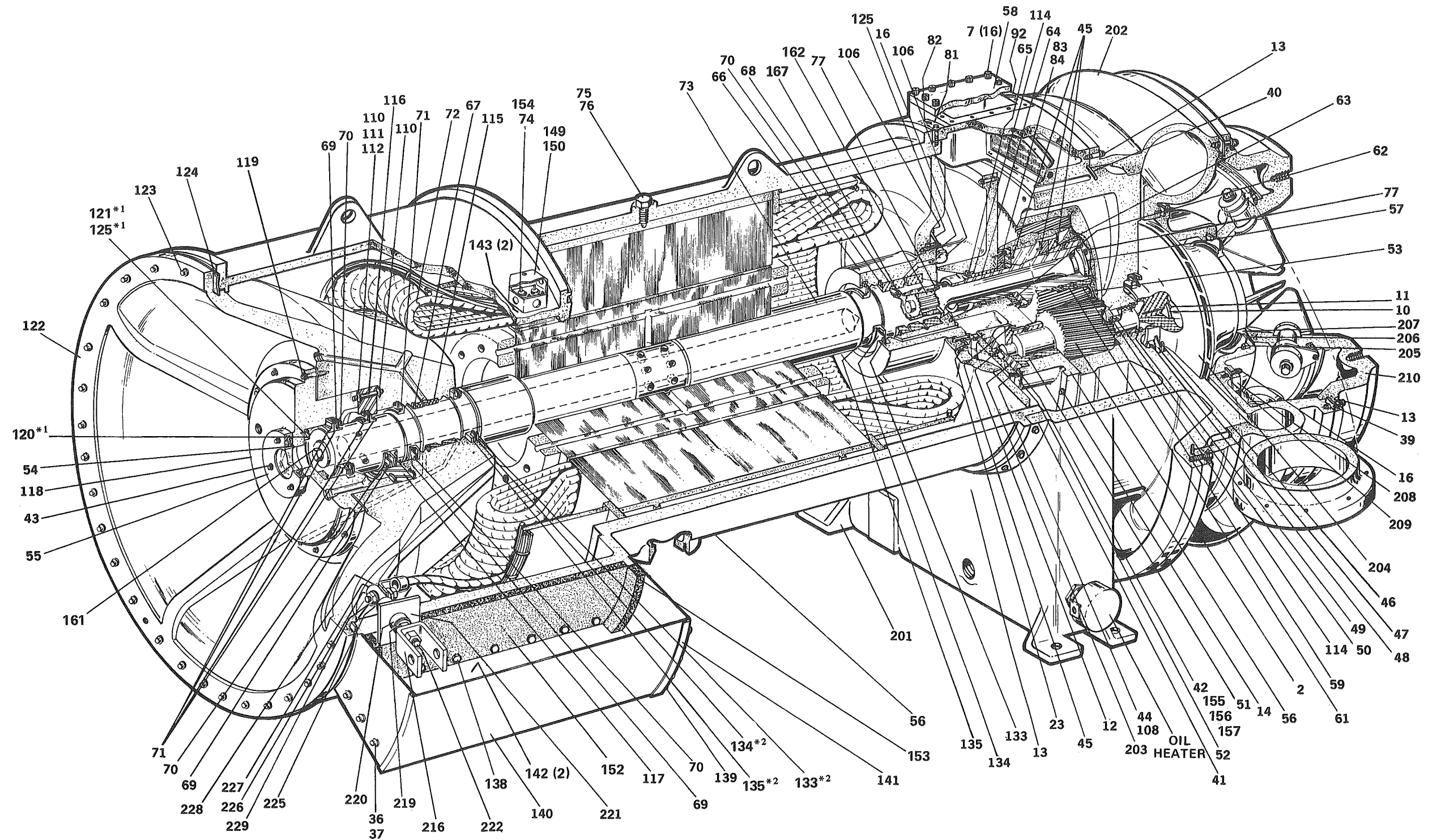
FIG. 2— MODEL MKB65 &amp; MKB73 COMPRESSORS, PARTS LOCATION
