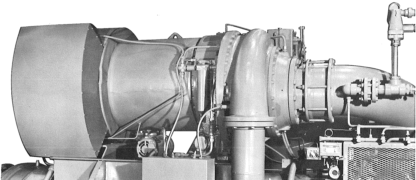
FIG. 1— HERMETIC—MOTOR COMPRESSOR, MODEL MKB
