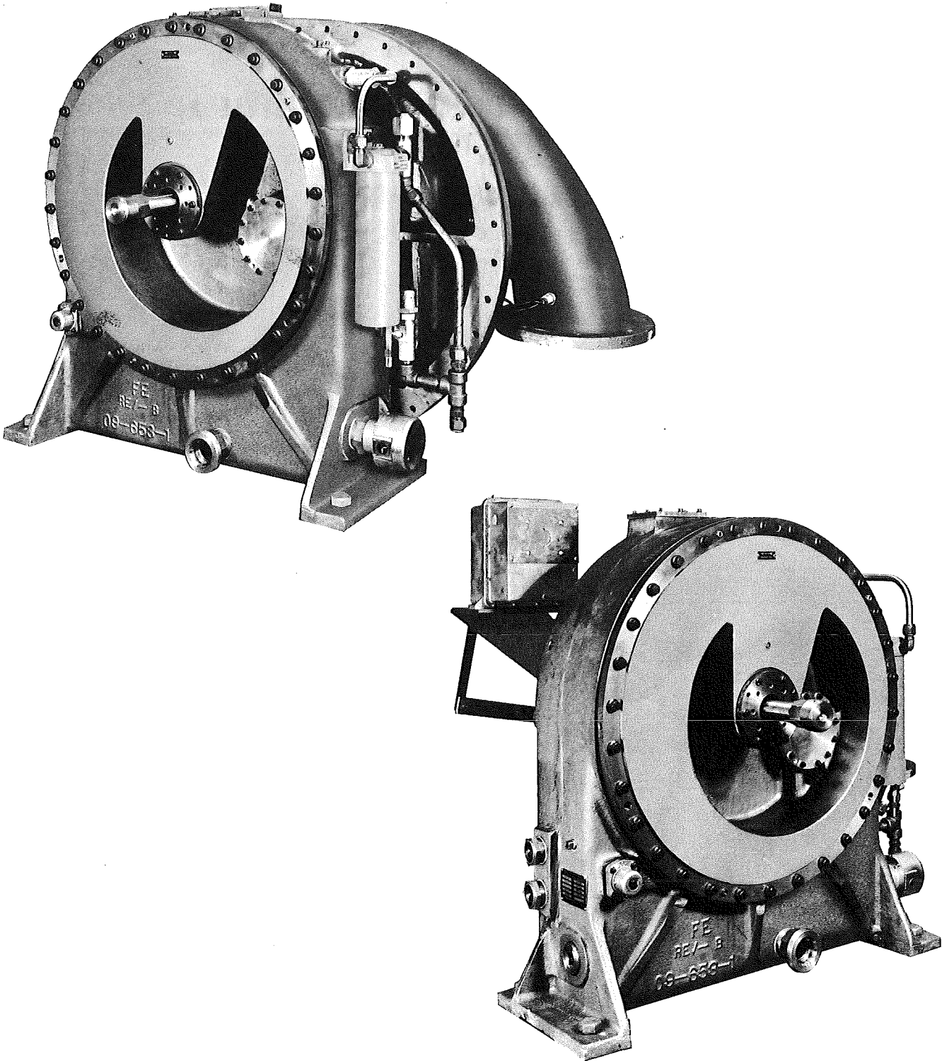
FIG. 1 – OPEN TYPE COMPRESSOR, MODEL LKA
