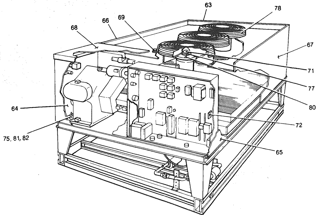
FIG. 4 - AIR COOLED WATER CHILLER
