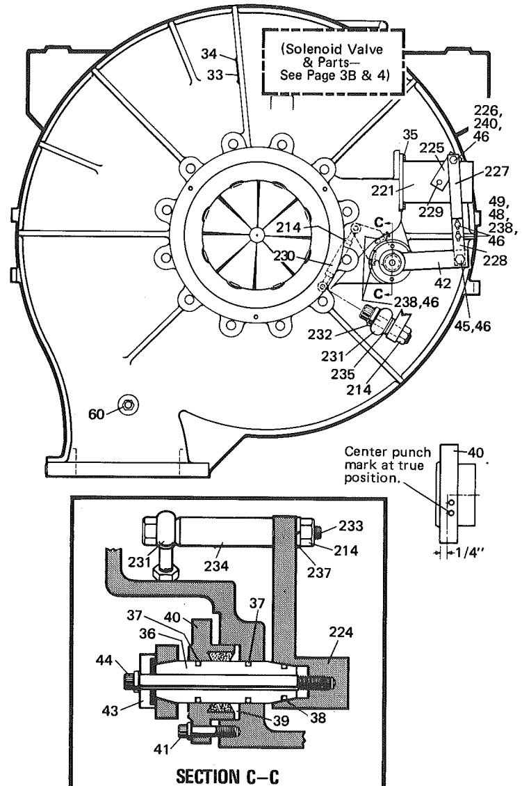
FIG. 4 — FRONT END VIEW MODELS YTJ & YDTJ 85-95 VANES IN CLOSED POSITION
