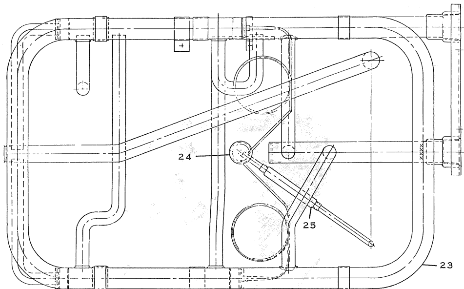
FIG. 8 — HC5W EVAPORATOR SECTION WITH CONNECTIONS
