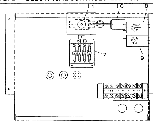
FIG. 3 — ELECTRICAL CONTROLS (208/220-3-60)
