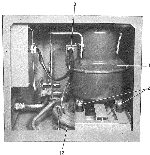
FIG. 1 — HC3W CHILLER UNIT
