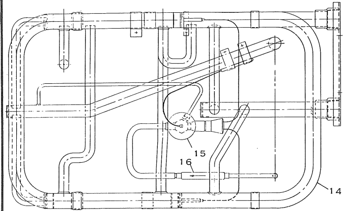
FIG. 5 — HC5A EVAPORATOR WITH CONNECTIONS
