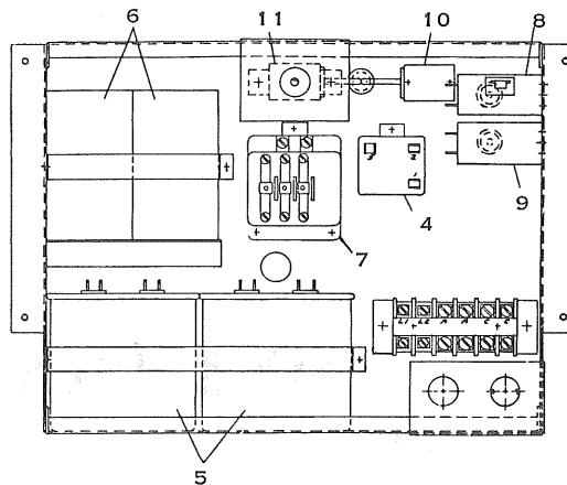
FIG. 2 — ELECTRICAL CONTROLS (230-1-60)
