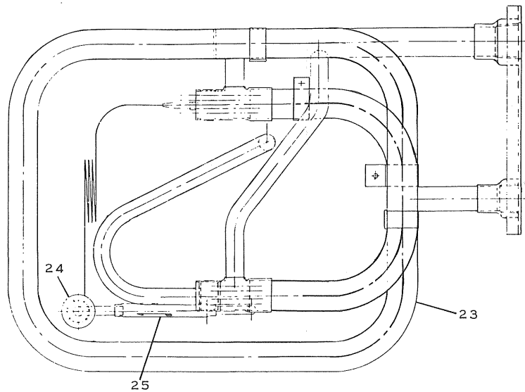
FIG. 7 — HC3W EVAPORATOR SECTION WITH CONNECTIONS
