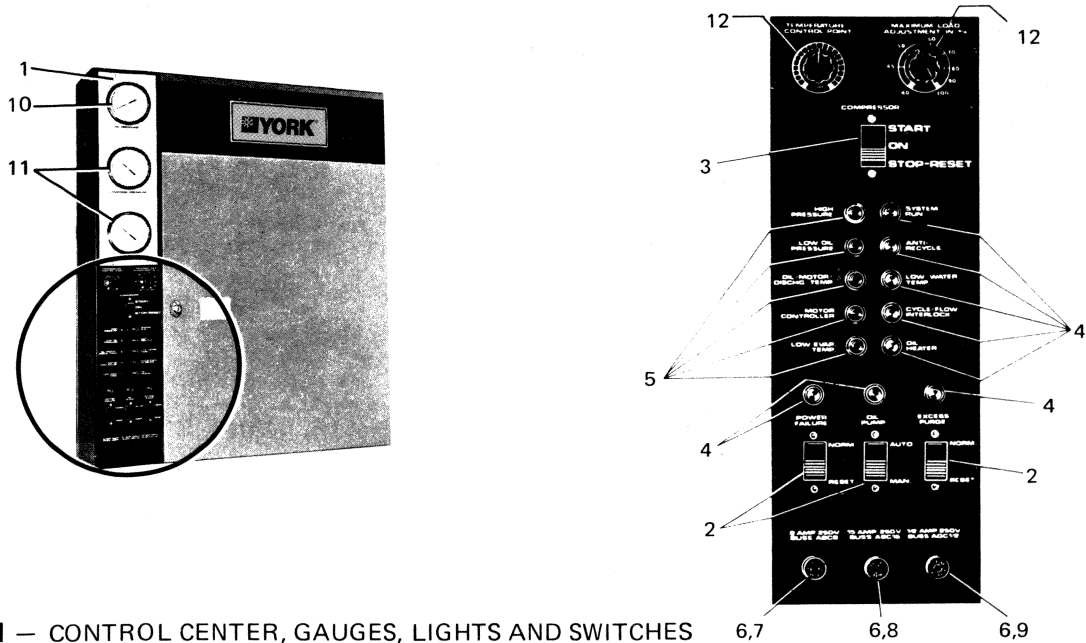
FIG. 1 — CONTROL CENTER, GAUGES, LIGHTS AND SWITCHES
