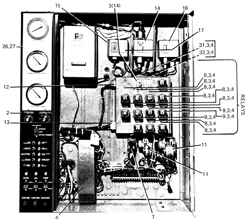
FIG. 3 — CONTROL CENTER
