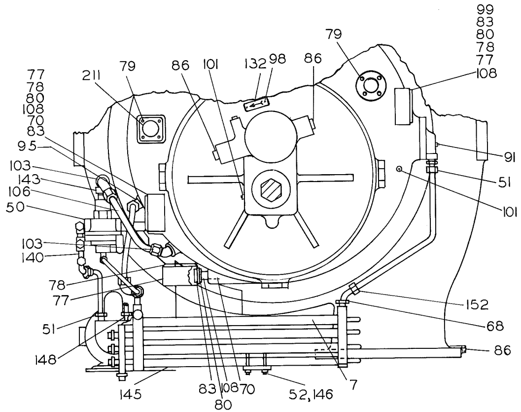
FIG. 2- Front View Compressor
